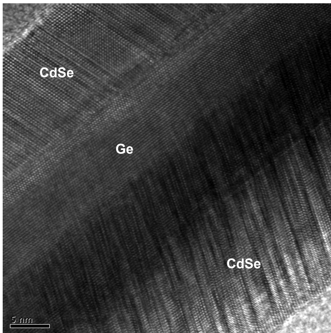
Fig. S1. HRTEM image of two interfaces in the sandwich-like triaxial nanowire between CdSe and Ge subnanowires. Both of the lower CdSe and the upper CdSe section have stacking defects
