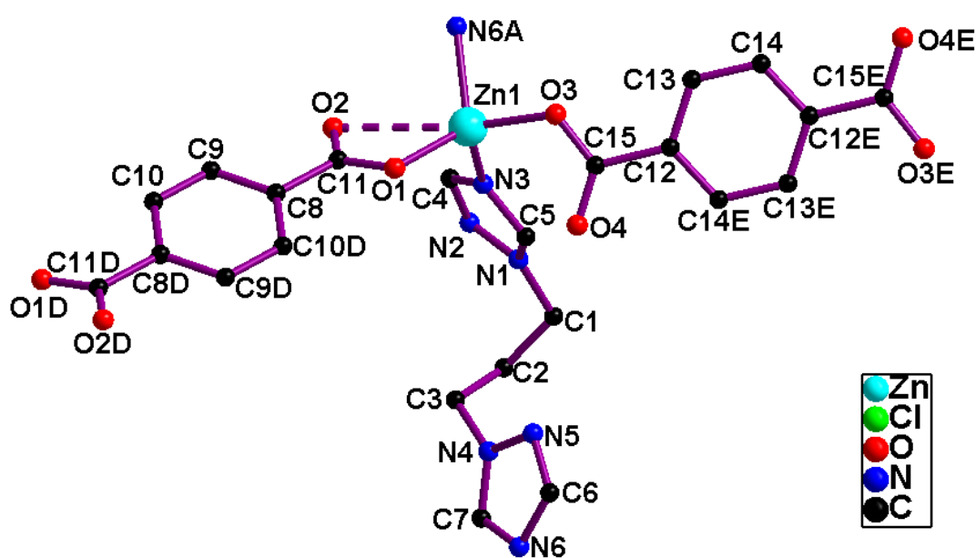
Fig. S1. The coordination environment of the Zn(II) ion of the (4,4) network in 1 .
