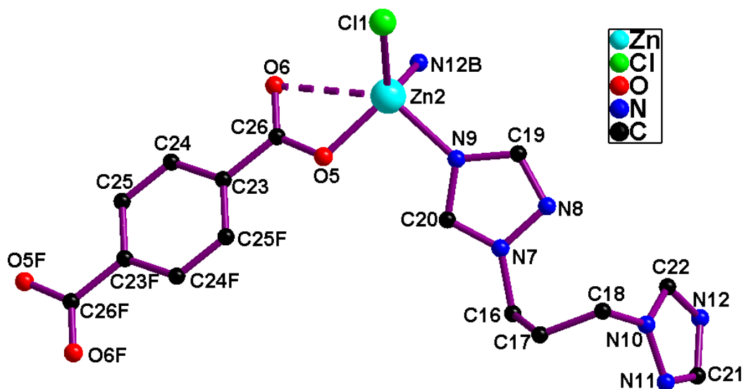
Fig. S2. The coordination environment of the Zn(II) ion of the 1D chain in 1.
