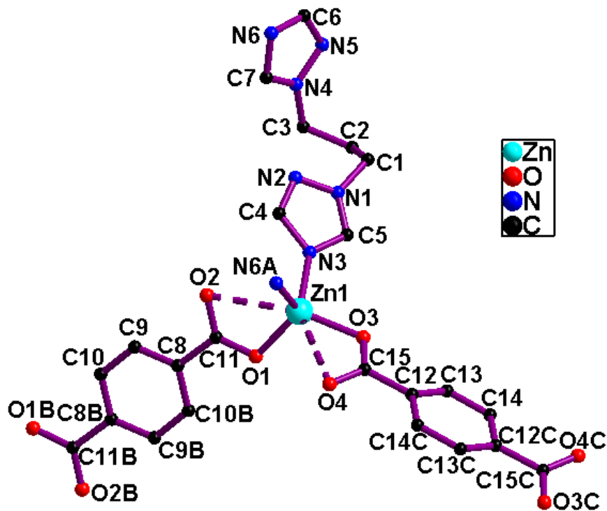
Fig. S3. The coordination environment of the Zn(II) ion in 2.
