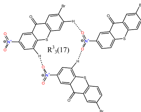
Compound 3 R^3_3(17)
