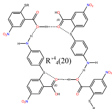
Compound 2 R'^4_4(20)
