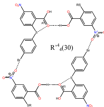
Compound 1 ( R'^4_4(30) )
