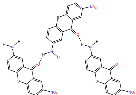
Compound 4
