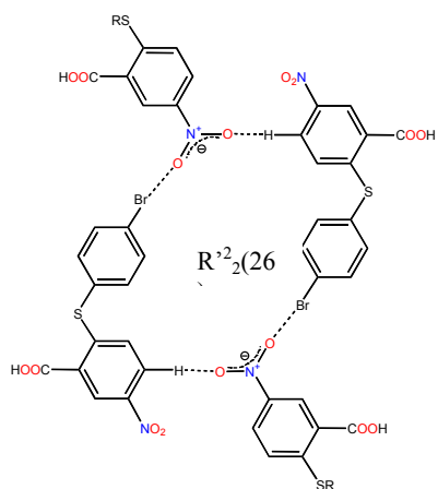
Compound 1 ( R'^2_2(26) )
