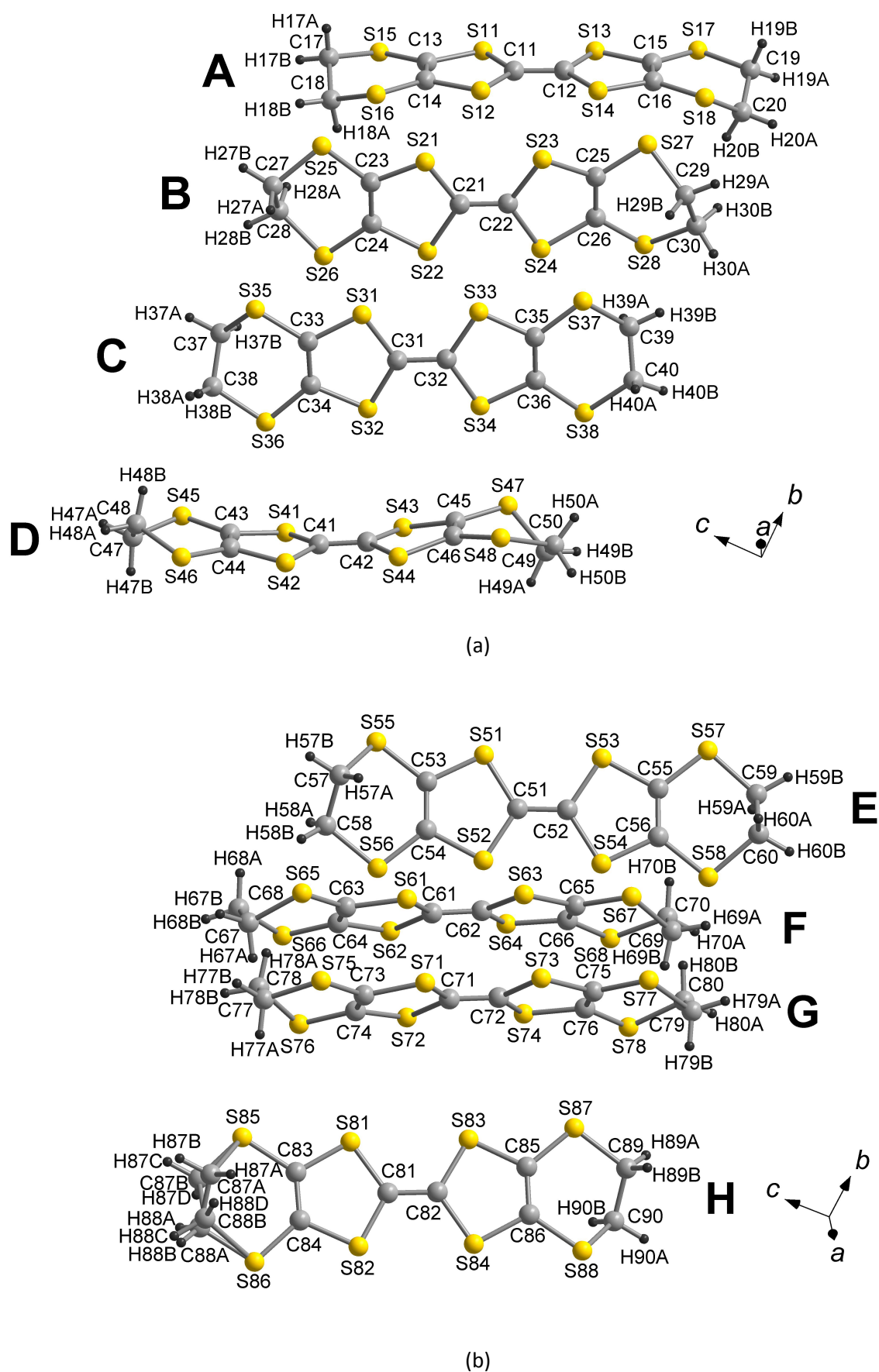
Fig. 2. Atom numbering scheme for the BEDT-TTF molecules in the 'pseudo- \kappa ' (a) and \alpha (b) conducting layers.
