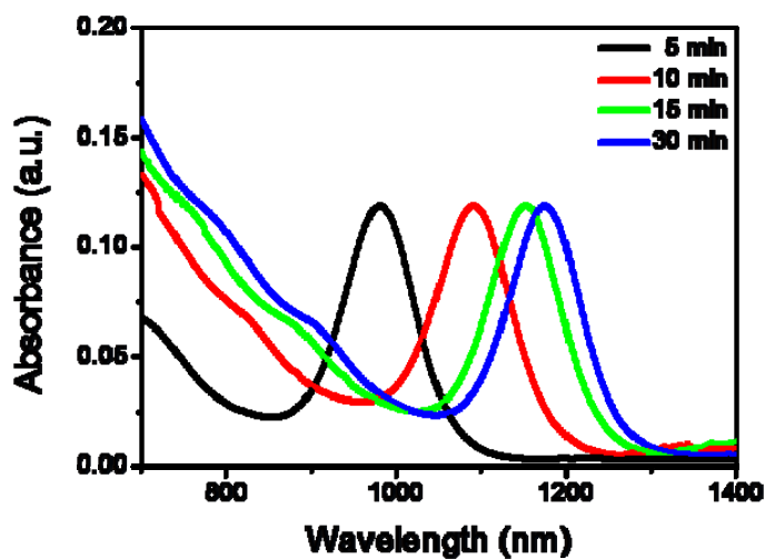
Fig. S1 Time evolution of the UV-vis-NIR absorption spectra during the PbS NC synthesis. Pb:S precursor molar ration is equal to 24:1.
