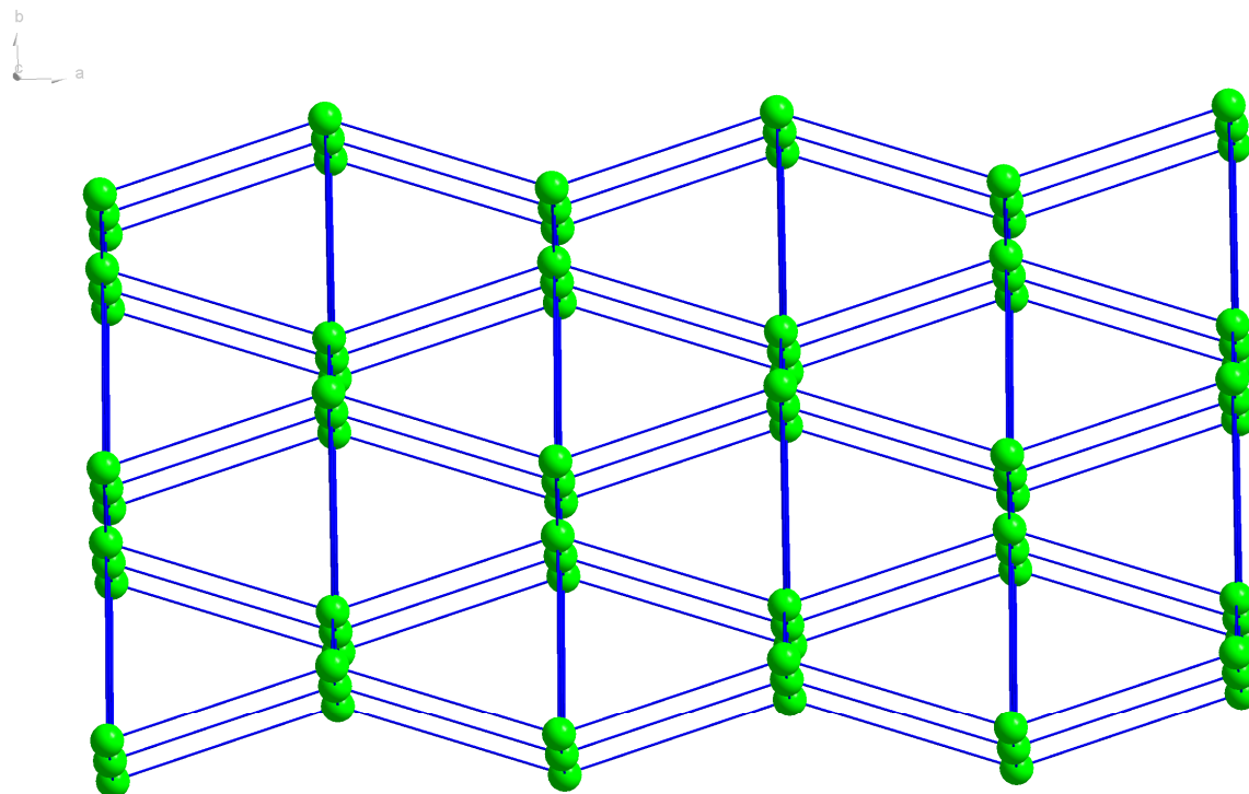
Fig. S1. A perspective view of 2 along the a direction revealing a peculiar 2D sheet framework
