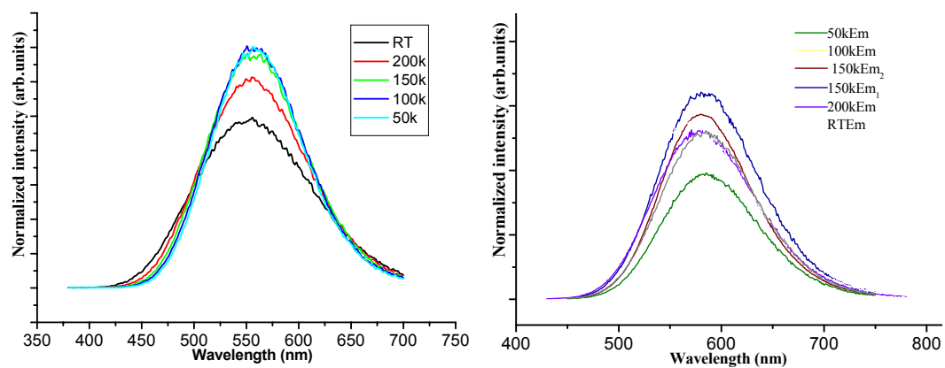
Fig. S6 The varied-temperature emission spectra of 1 (left) and 2 (right)
