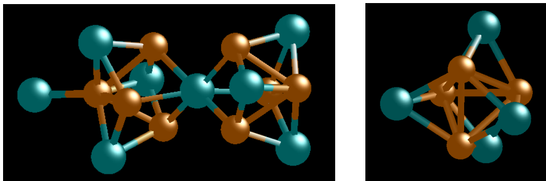
Fig. S5 The stoichiometry-discriminated assemblies of ICCs of 1 (left) and 2 (right)
