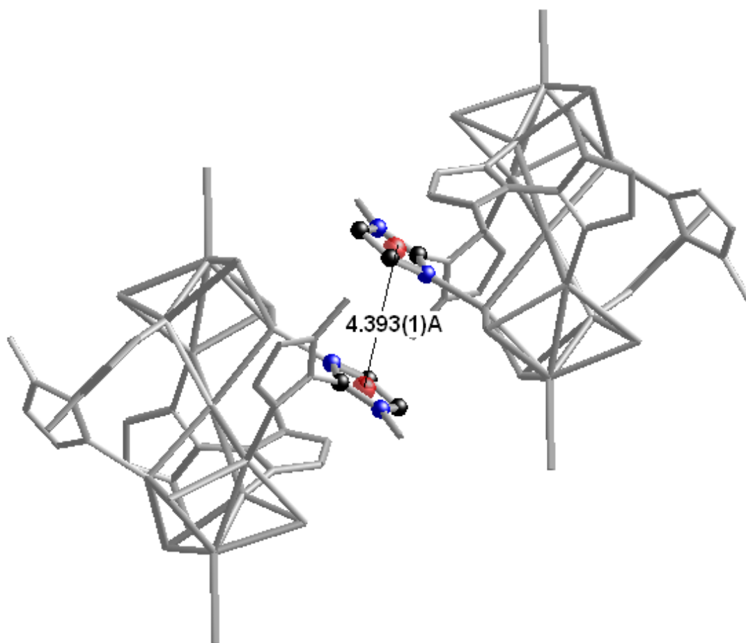
Fig. S3 The parallel \pi - \pi interaction presenting among the entities of 1
