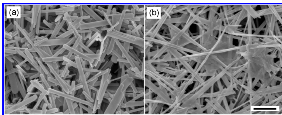
Fig. S2. SEM images of VO 2 (B) nanostructures obtained at volume ratio between polyethylene glycol and V 2 O 5 sol of (a) 2:3 and (b) 7:3. The scale bar is 2 μm.
