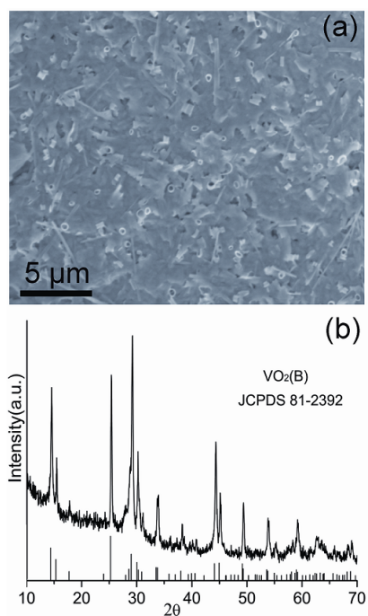
Fig. S1. (a) A low-magnification SEM image of VO 2 (B) nanorings and (b) the corresponding powder XRD pattern.
