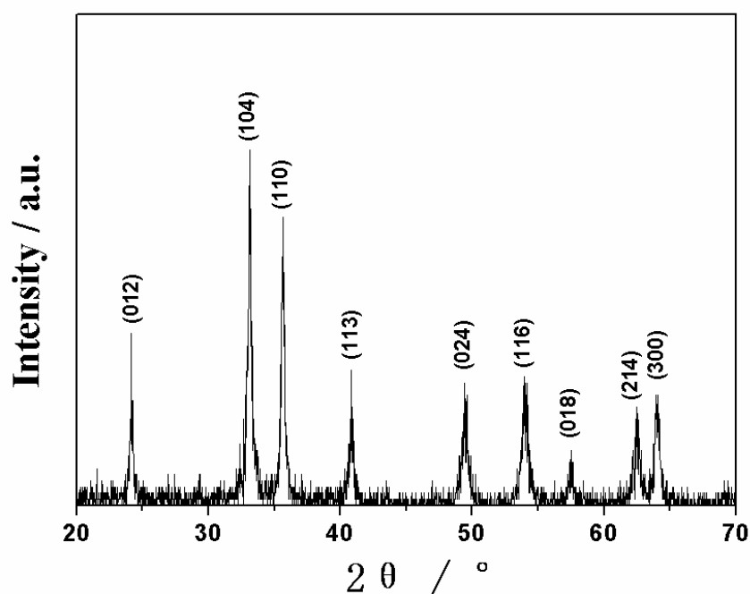
Fig. S1 XRD pattern of the sample after solvothermal reaction.
