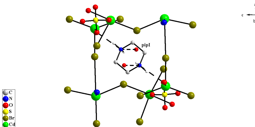
Fig. S2 The 2-D supramolecular sheet constructed up from the 1-D tube by the intermolecular hydrogen bondings in compound 1.
