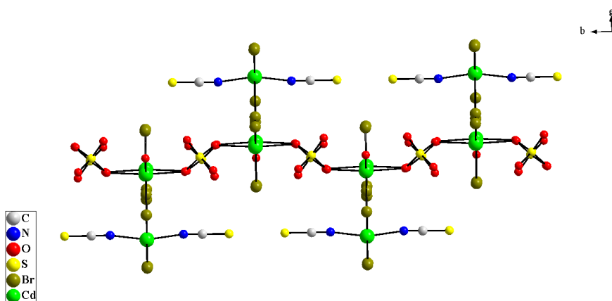
Fig. S1 Two such parallel chains extend along the b -axial direction, and the Cd1 octahedra sit alternately above and below the plane of the two chains in compound 1.
