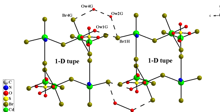
Fig. S2 The 2-D supramolecular sheet constructed up from the 1-D tube by the intermolecular hydrogen bondings in compound 1.
