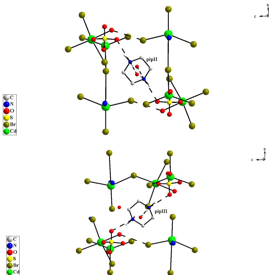
Fig. S3 The N-H \cdots O( \text{SO}_4^{2-} ) hydrogen bonds between the \text{H}_2\text{pip}^{2+} cations and the host frameworks, and the N-H \cdots Ow hydrogen bonds between the \text{H}_2\text{pip}^{2+} cations and the lattice \text{H}_2\text{O} molecules in compound 1 .
