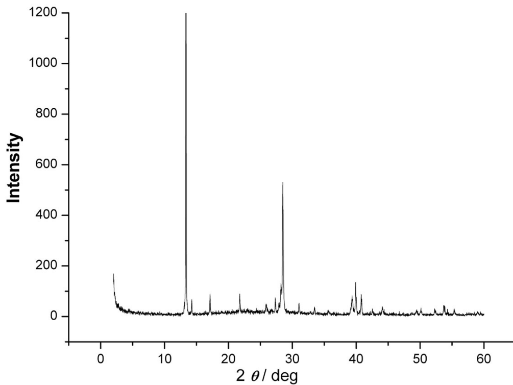
Figure S-3: XRPD of the compound with unknown structure obtained by reaction of \text{Cd}(\text{OAc})_2 \cdot 2\text{H}_2\text{O} with Hnim.
