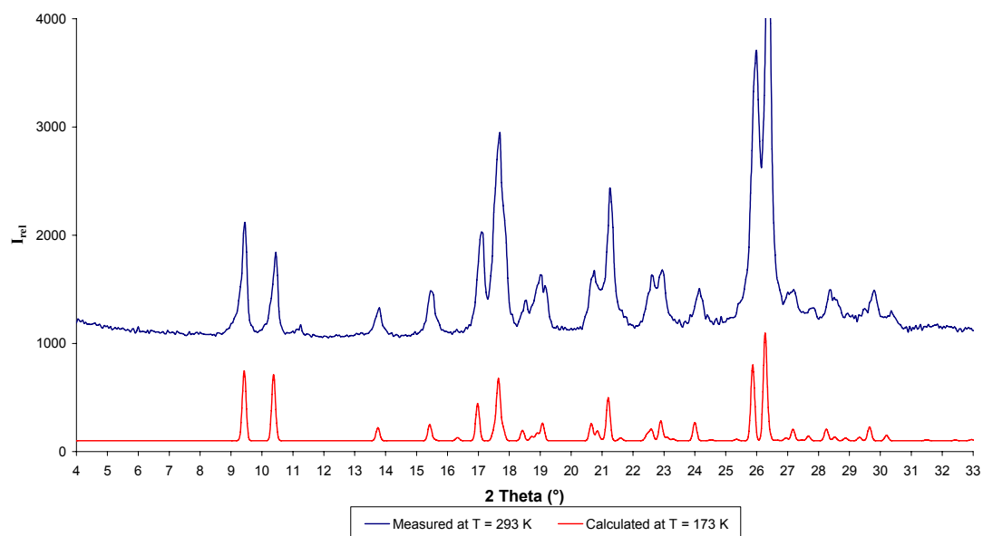
Figure S4. Comparative calculated and measured PXRD pattern for 7 .
