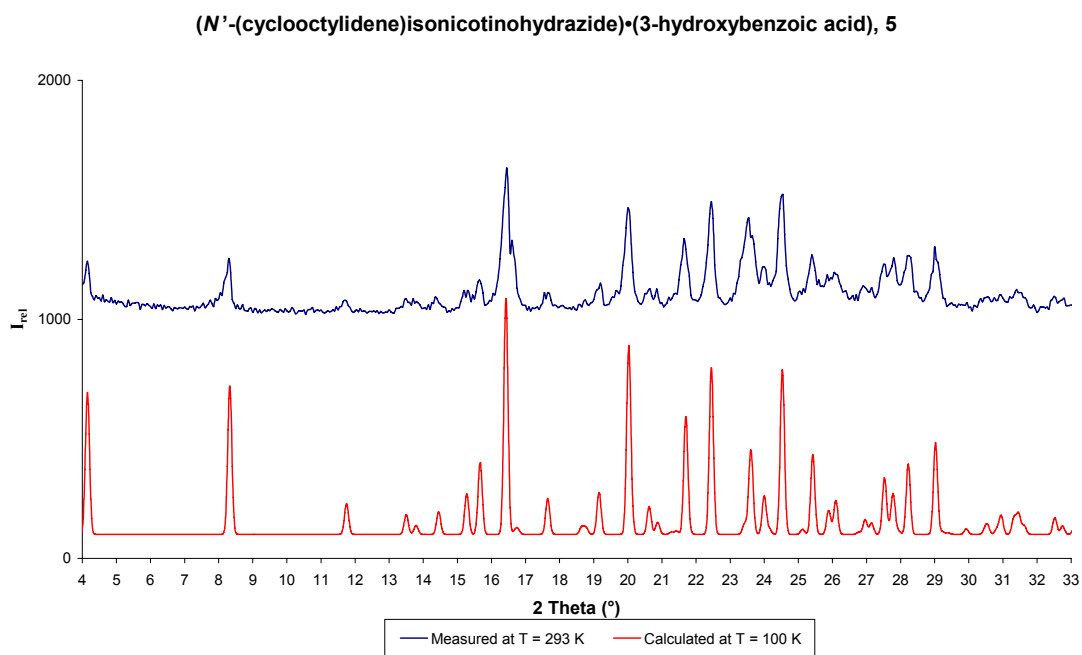
Figure S2. Comparative calculated and measured PXRD pattern for 5 .
