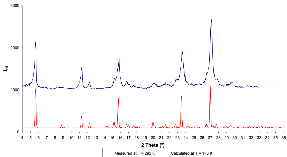
Figure S9. Comparative calculated and measured PXRD pattern for 12 .
