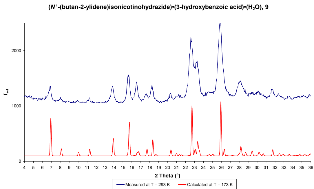
Figure S6. Comparative calculated and measured PXRD pattern for 9 .
