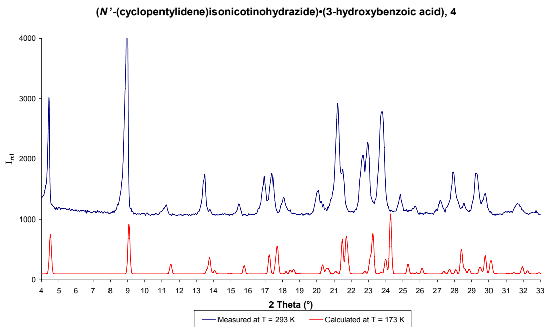
Figure S1. Comparative calculated and measured PXRD pattern for 4 .
