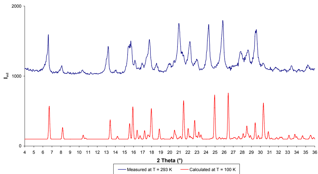
Figure S7. Comparative calculated and measured PXRD pattern for 10 .
