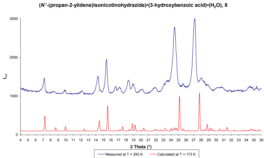
Figure S5. Comparative calculated and measured PXRD pattern for 8 .
