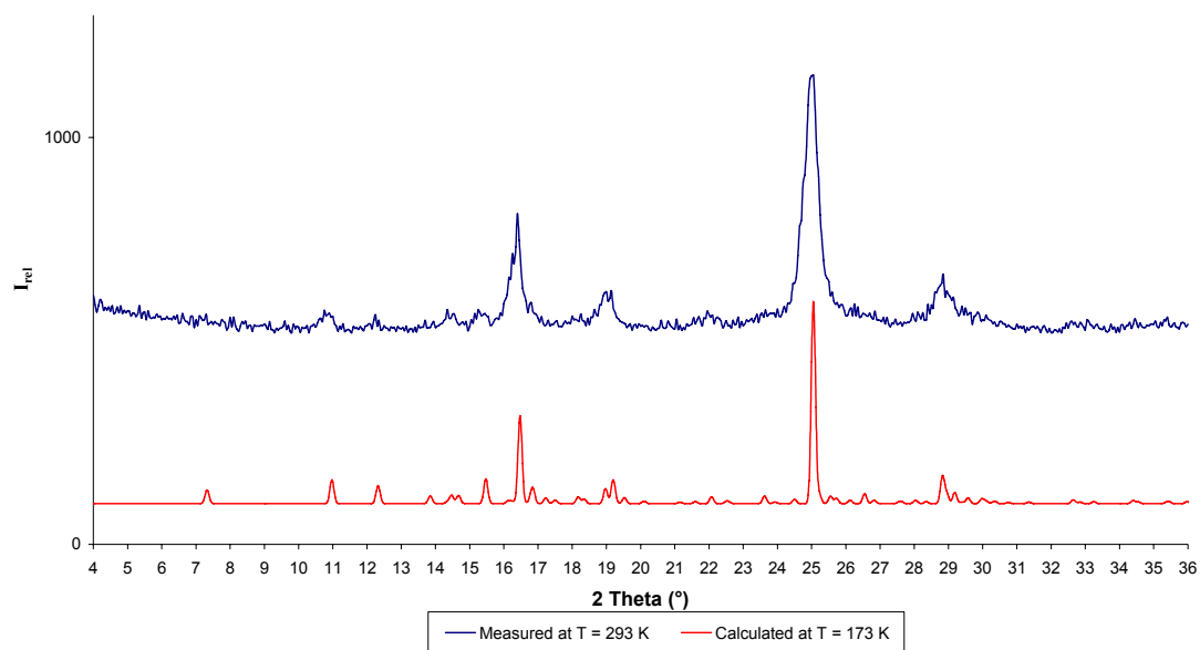
Figure S3. Comparative calculated and measured PXRD pattern for 6 .
