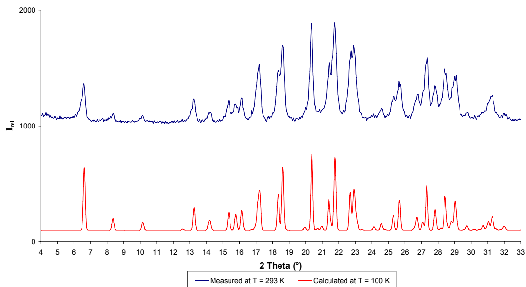
Figure S8. Comparative calculated and measured PXRD pattern for 11 .
