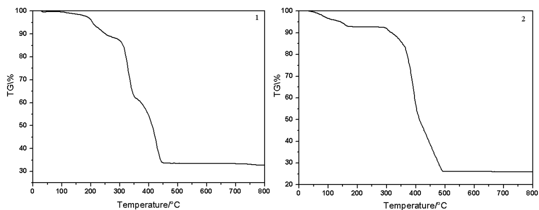
Figures. S1~S2 TGA curves for 1 and 2 , respectively.
