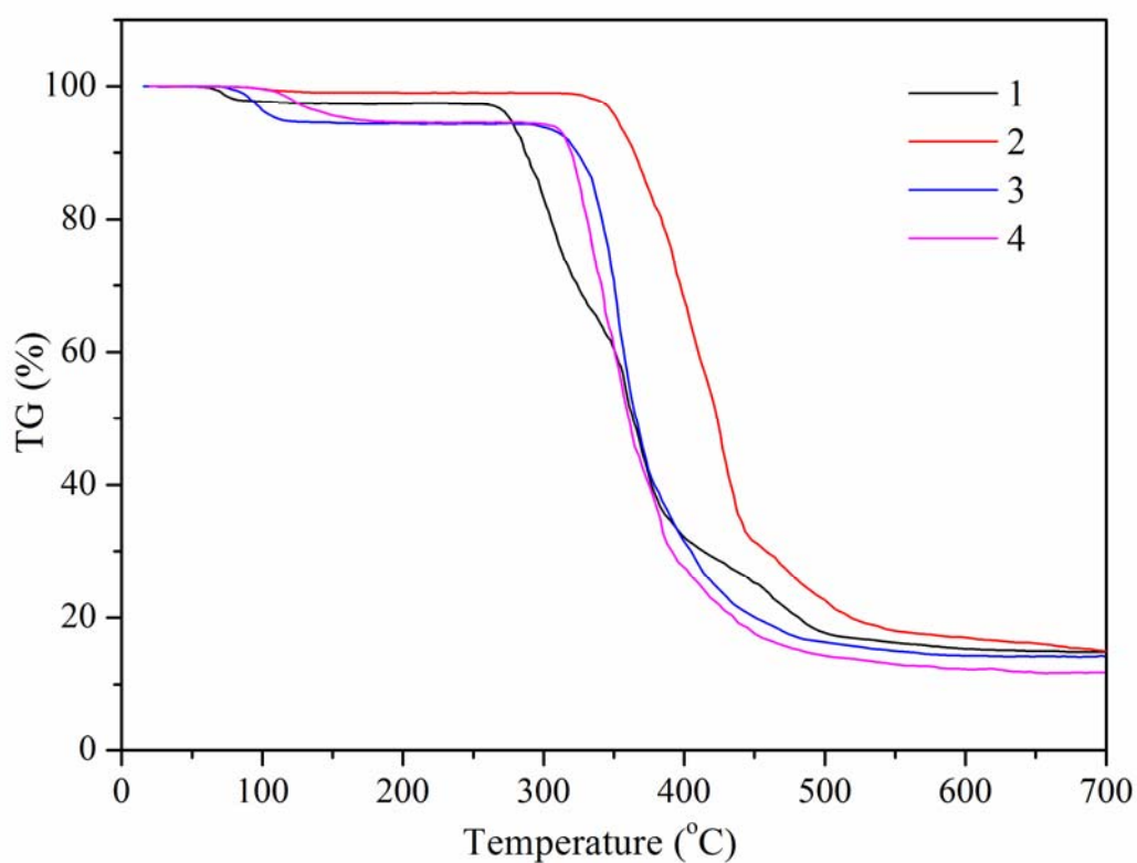
Fig. S1. TGA curves for complexes 1-4 under nitrogen atmosphere.
