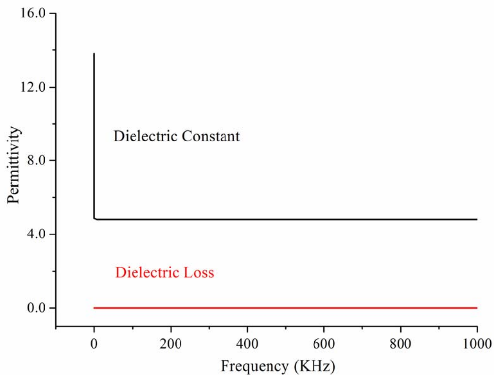
Fig. S2 Frequency dependence of permittivity ( \epsilon = \epsilon_1(\omega) - i\epsilon_2(\omega) ) of complex 1 at room temperature (20°C).
