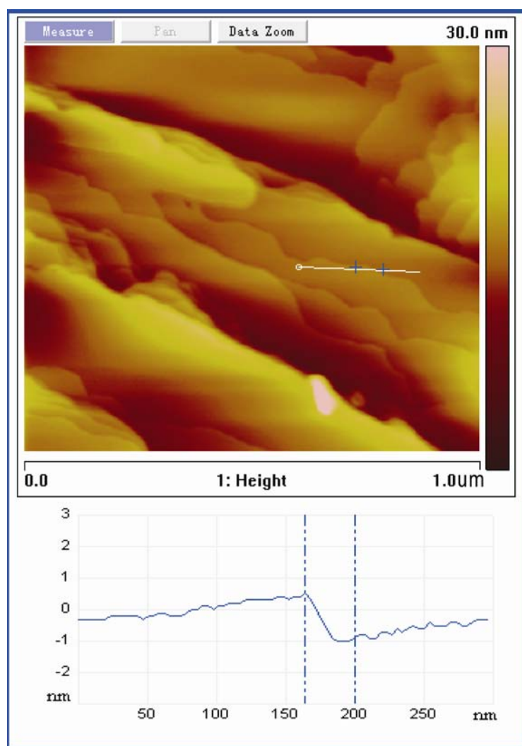
Figure S2. The AFM image of the layered structure of L-leucine crystal surface.
