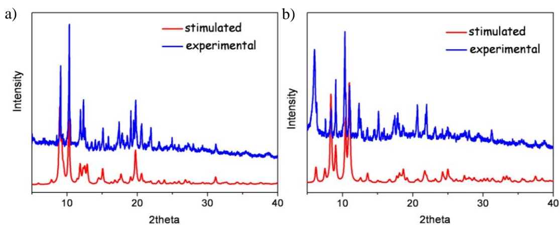
Figure S1. The XRD spectra of 1 (a) and 2 (b).
