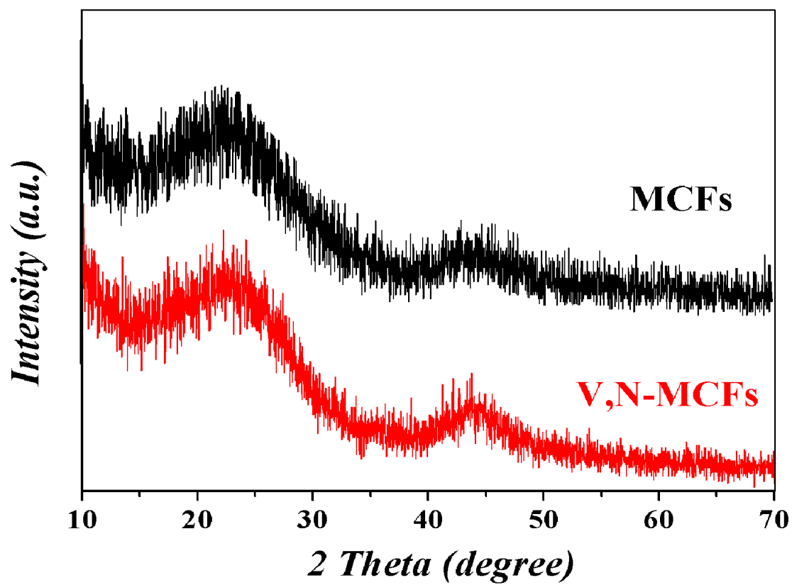
Fig. S3. Wide-angle XRD patterns of V, N-MCFs and MCFs.
