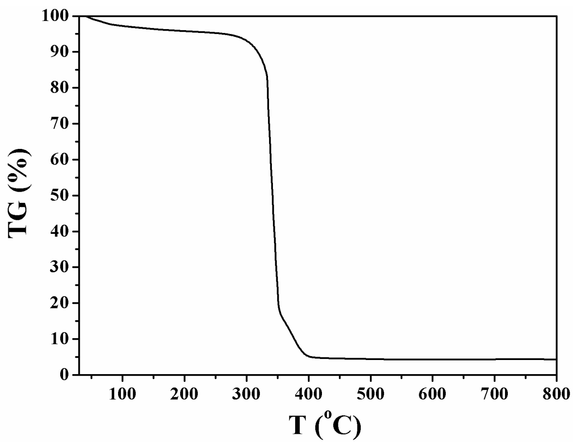
Fig. S2 TG curve of V, N-MCFs under air atmosphere.
