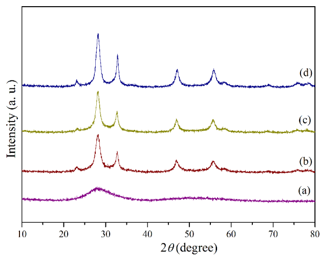
Supporting Information, Fig. S2. XRD patterns of the products collected at different time intervals with the aid of 0.40 g EDTA. (a) 1 h, (b) 4 h, (c) 9 h, and (d) 12 h.
