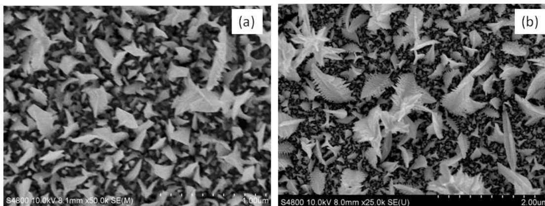
Figure S1 (a): Morphology of gold deposited on p-type silicon in presence of green laser. Irregular morphology with dendritic features is observed. (b) In presence of red laser wherein flat dendrites are observed
