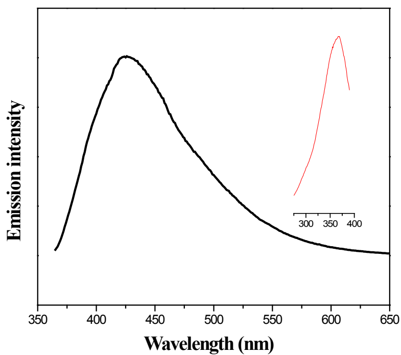
Fig. S2 Emission spectrum and excitation spectrum (inset) of Bime.
