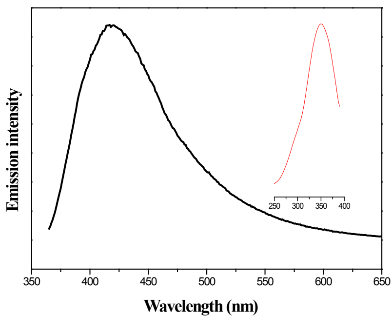
Fig. S3 Emission spectrum and excitation spectrum (inset) of Bimb.
