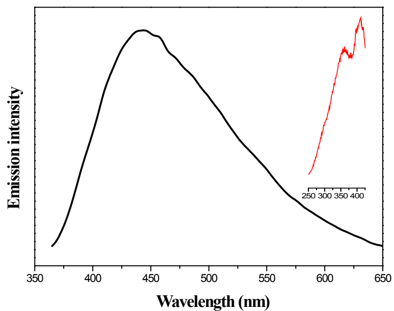
Fig. S1 Emission spectrum and excitation spectrum (inset) of Bpmb-2HBr.
