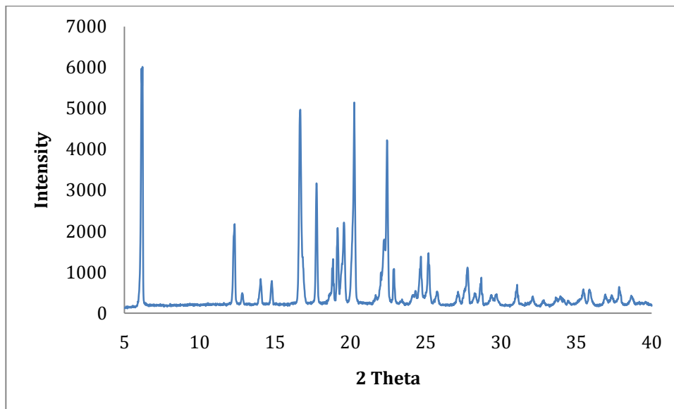
Figure 1 X-ray Powder Diffraction of IBU
