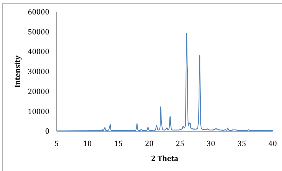
Figure 3 X-ray Powder Diffraction of BIPY
