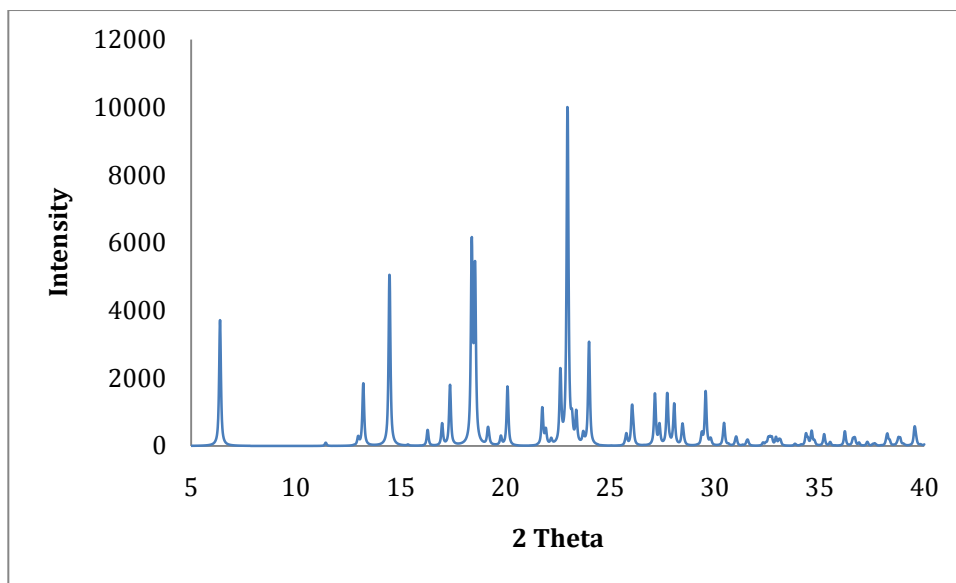
Figure 2 X-ray Powder Diffraction of KETO
