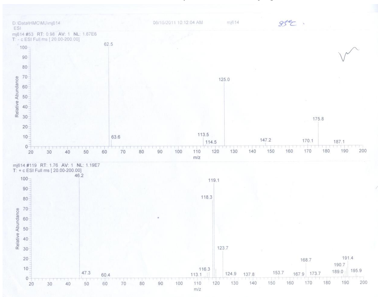
Figure S1. ESI mass spectrum of mother solution of 1 .
