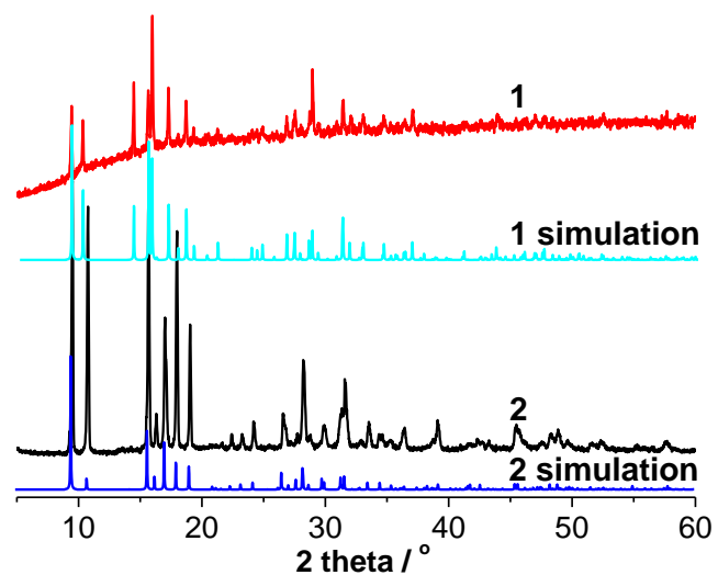
Fig. S1 XRD patterns for compounds 1 and 2 .
