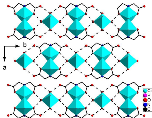
Fig. S3 Packing diagram of structure 1 along the c -axis.
