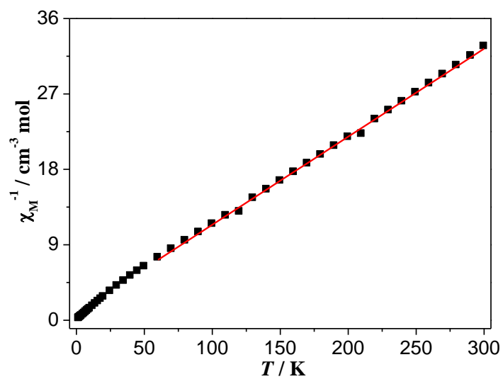
Fig. S5 The \chi_M^{-1} versus T plot for 1 .
