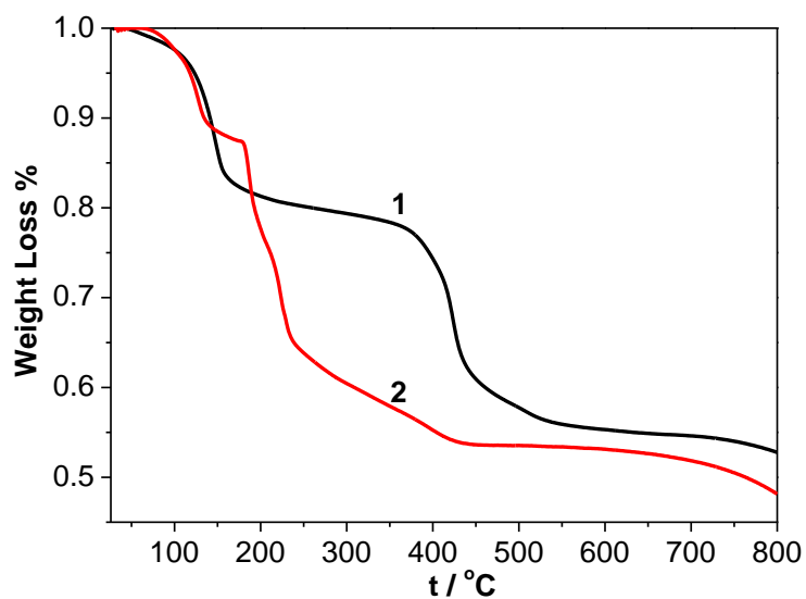
Fig. S2 TG curves for compounds 1 and 2 .
