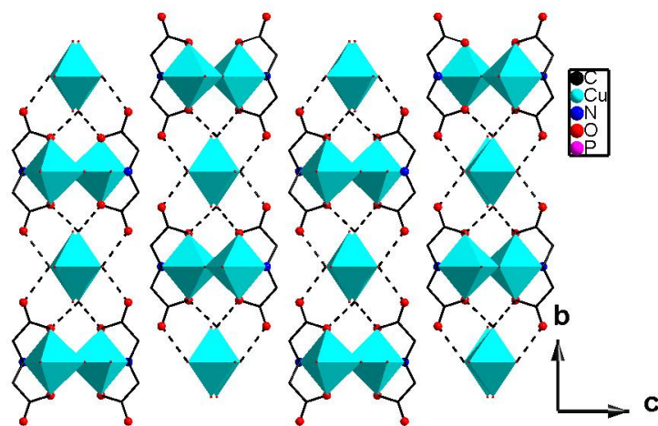
Fig. S4 Packing diagram of structure 2 along the a -axis.
