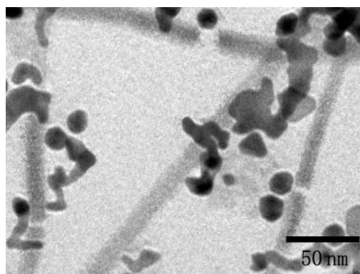
Fig.SI2. Typical TEM image of Au microstructures for the first case..
