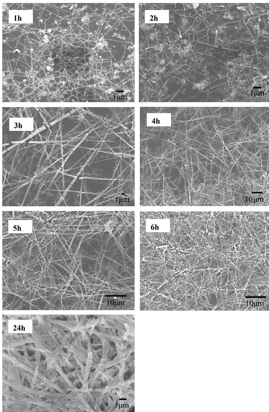
Fig. S11. Typical SEM images of Au microstructures on the silicon substrate at different growth times for the first case.
