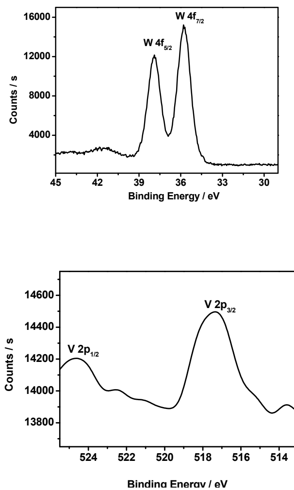
Fig. SI3. XPS spectra of the Au microstructures of W 4f and V 2p at \gamma = 10 .
