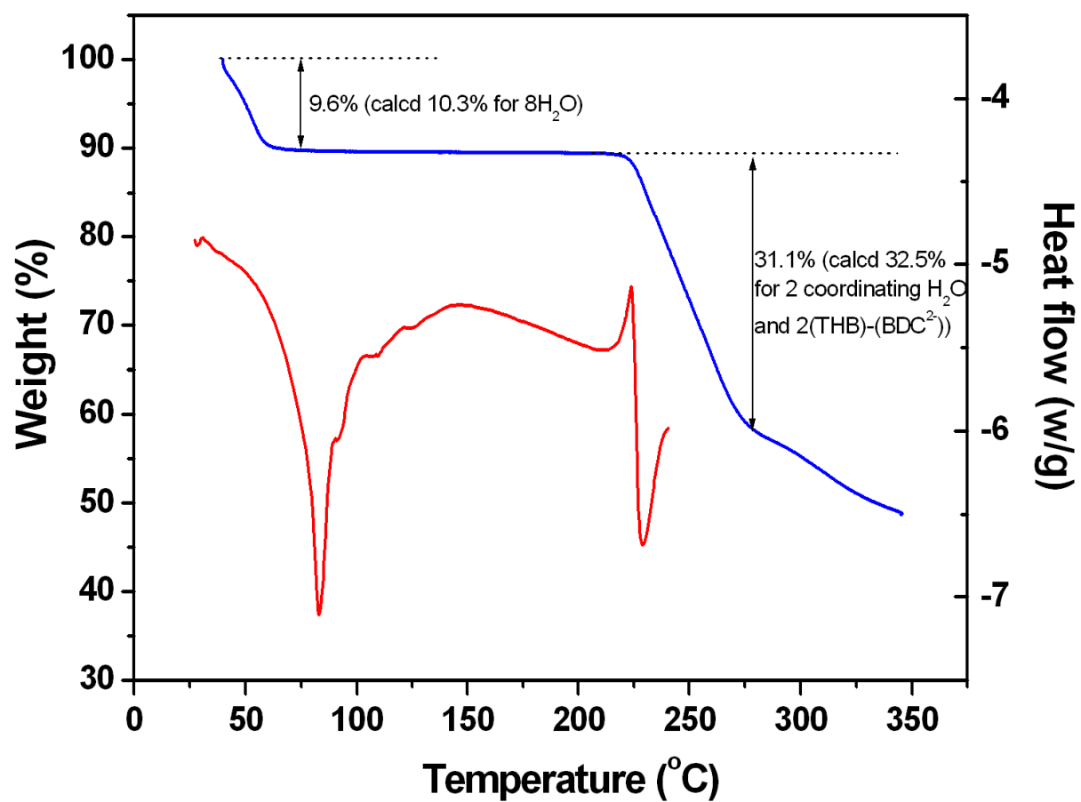
Figure S4. TGA/DSC trace for 4.
