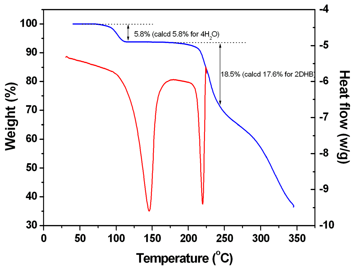
Figure S2. TGA/DSC trace for 2.
