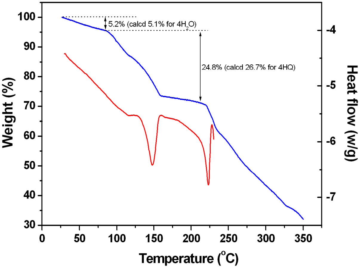
Figure S3. TGA/DSC trace for 3.
