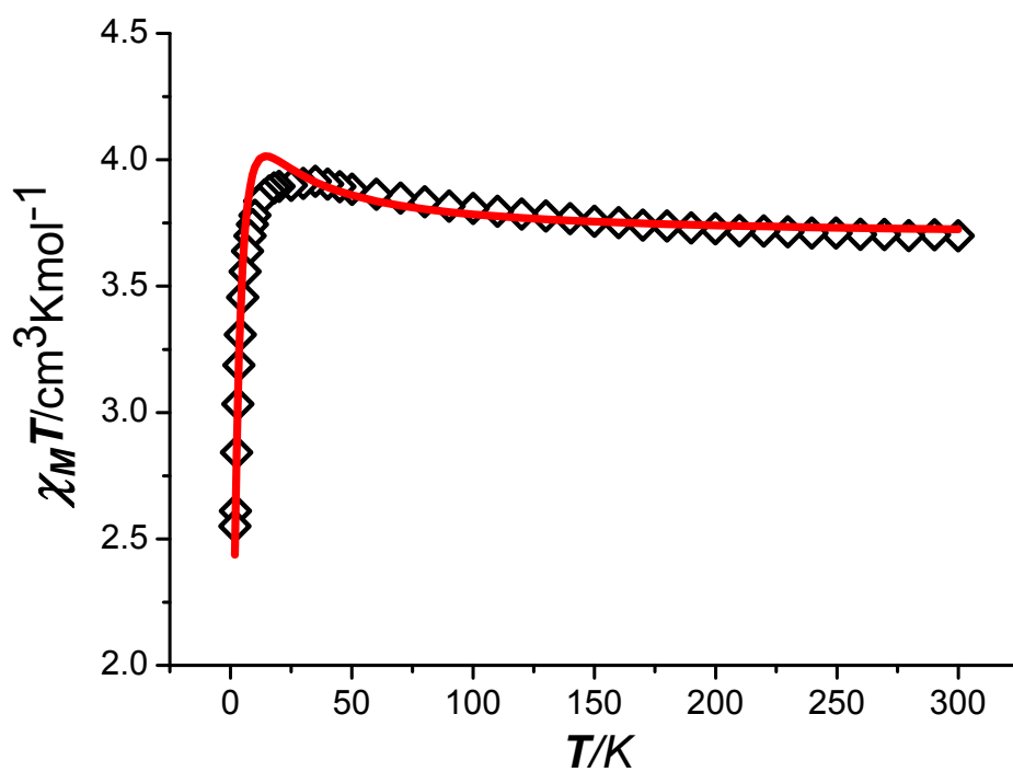
Figure S2 The fitting curve of \chi T without zero-field splitting for polymorph 2.
