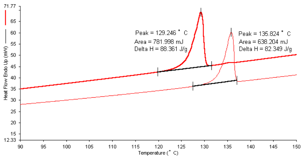
Fig. S3 DSC curves of polymorphs A and B
