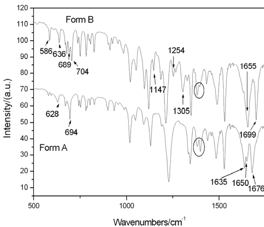
Fig. S1 FT-IR spectra of polymorphs A and B
