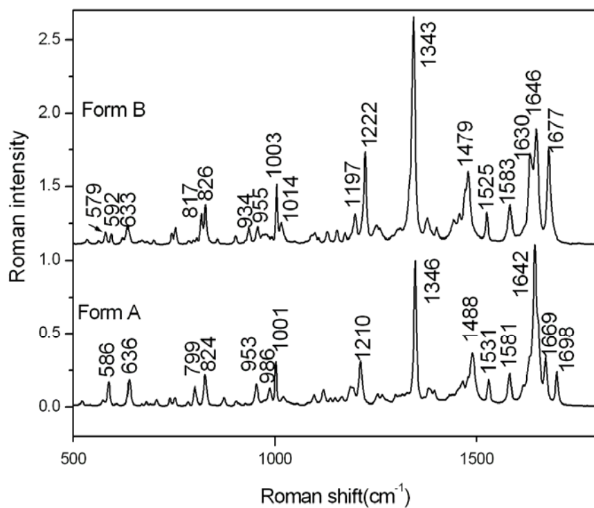
Fig. S2 Raman spectra of polymorphs A and B
