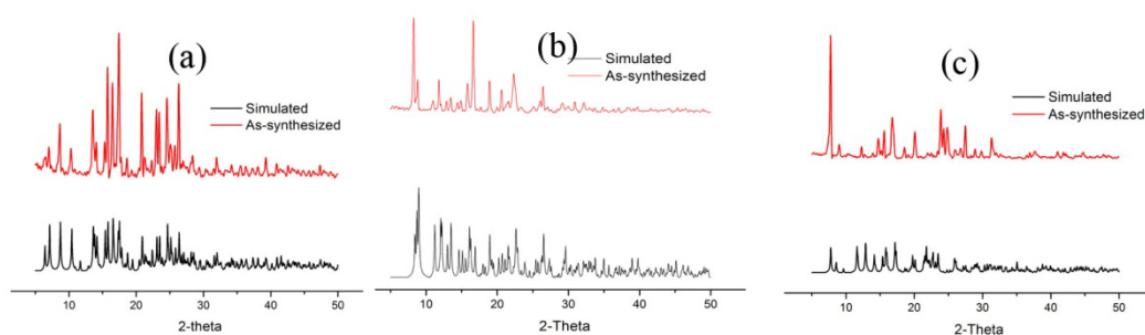
Figure S2. Comparison of XRPD patterns of the simulated pattern from the single-crystal structure determination for compounds 1-3 (order of a-c).
