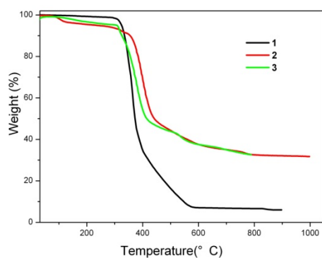
Figure S1. The diagram of TGA for complexes 1-3
