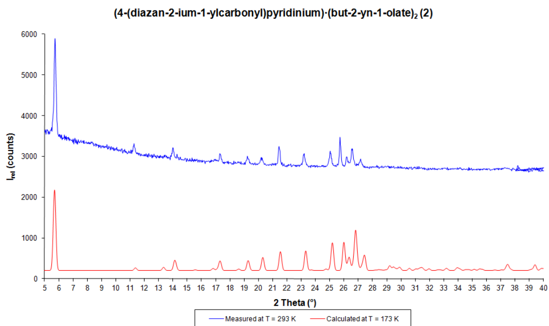
Figure S2. Comparative calculated and measured PXRD pattern for 2 .
