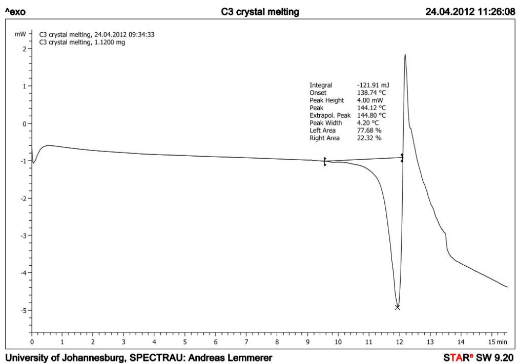
Figure S3. DSC trace for salt 1.
