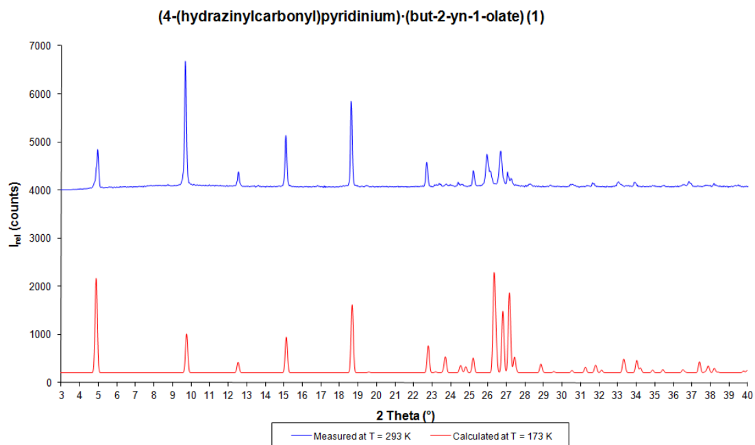
Figure S1. Comparative calculated and measured PXRD pattern for 1 .
