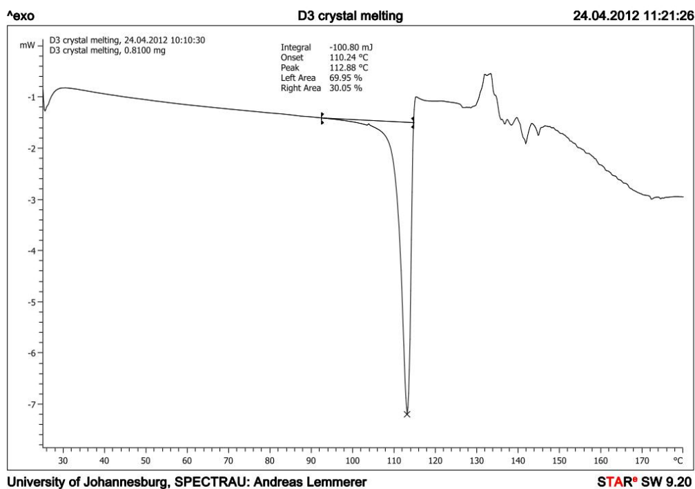
Figure S4. DSC trace for salt 2.
