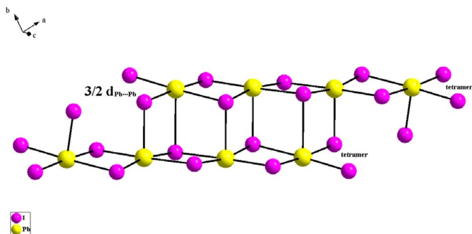
Fig. S1 The packing pattern of the adjacent tetramers in compound 2.
