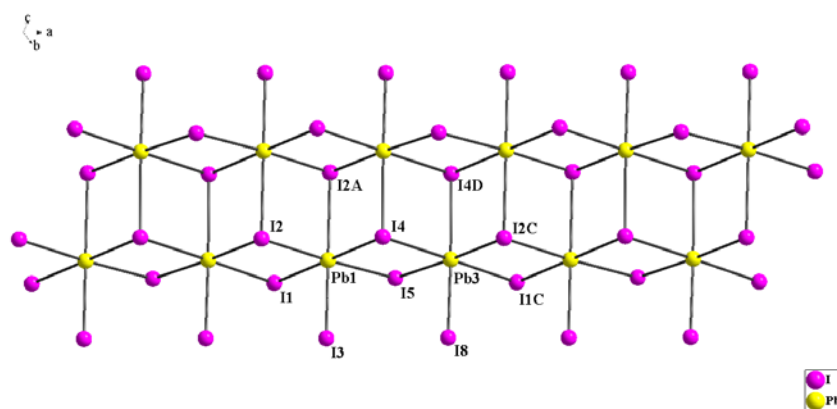
Fig. S2 The 1-D ribbon in compound 3.
