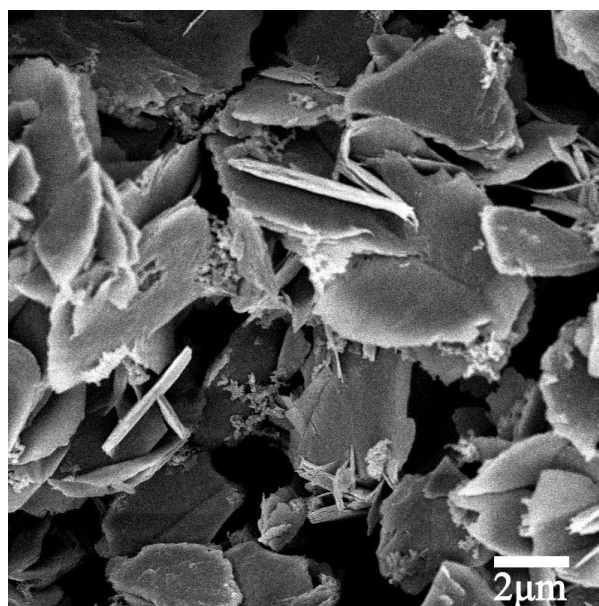
Fig. S1 SEM image of LFP sample synthesized with 5 wt% TiO 2 nanoparticle addition.
