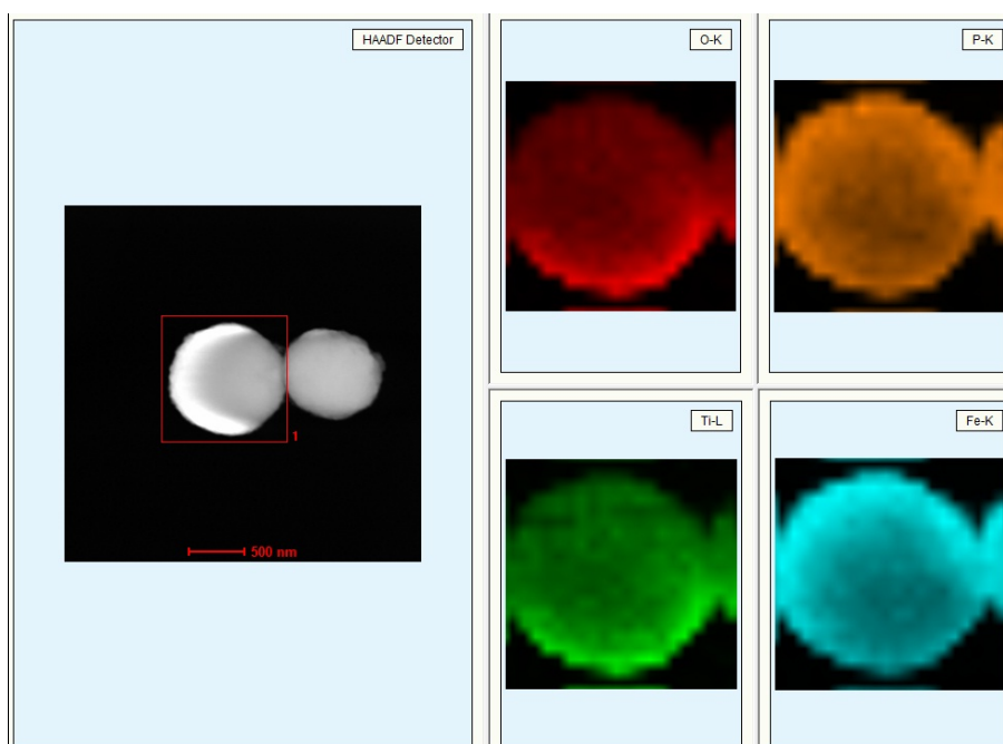
Fig. S2 EDS mapping of O, P, Fe and Ti of a single LiFePO 4 microsphere.
