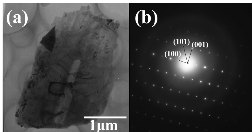
Fig. S3 TEM and SEAD images of \text{LiFePO}_4 sample synthesized in the absence of TiN.
