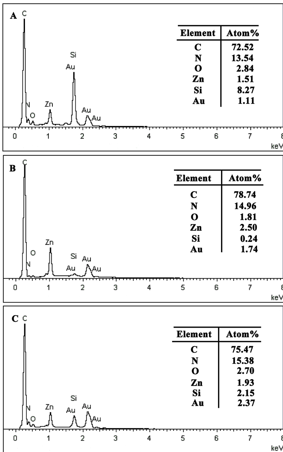
Fig. S3 The energy dispersed X-ray (EDX) images of micro-prisms (A), micro-octahedrons (B), and self-assembled ZnTPyP micro-rods (C).
