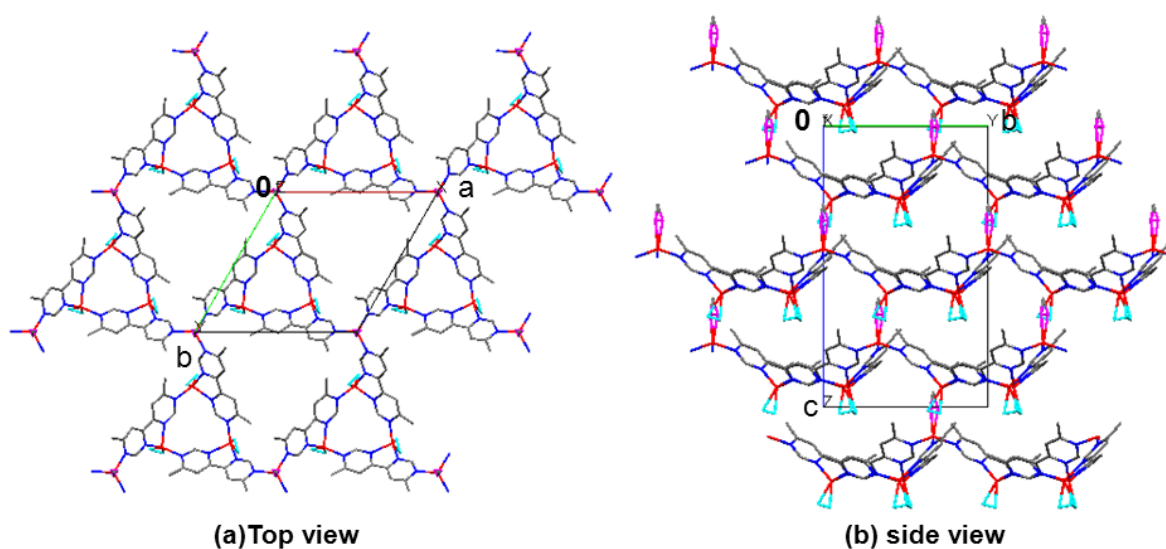
Fig. S-1 X-ray crystal packing structures of complex 3 along c-axis (a) and a-axis (b). The encapsulating ClO 4 - anions were omitted for clarity.
