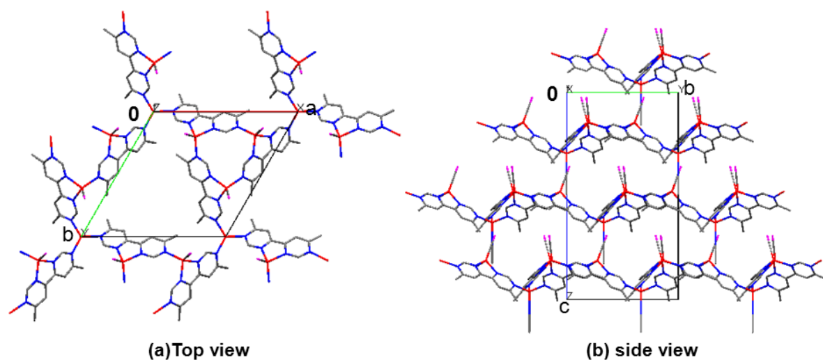
Fig. S-2 X-ray crystal packing structures of complex 4 along c-axis (a) and a-axis (b). The encapsulating MeCN and \text{PF}_6^- anions were omitted for clarity.
