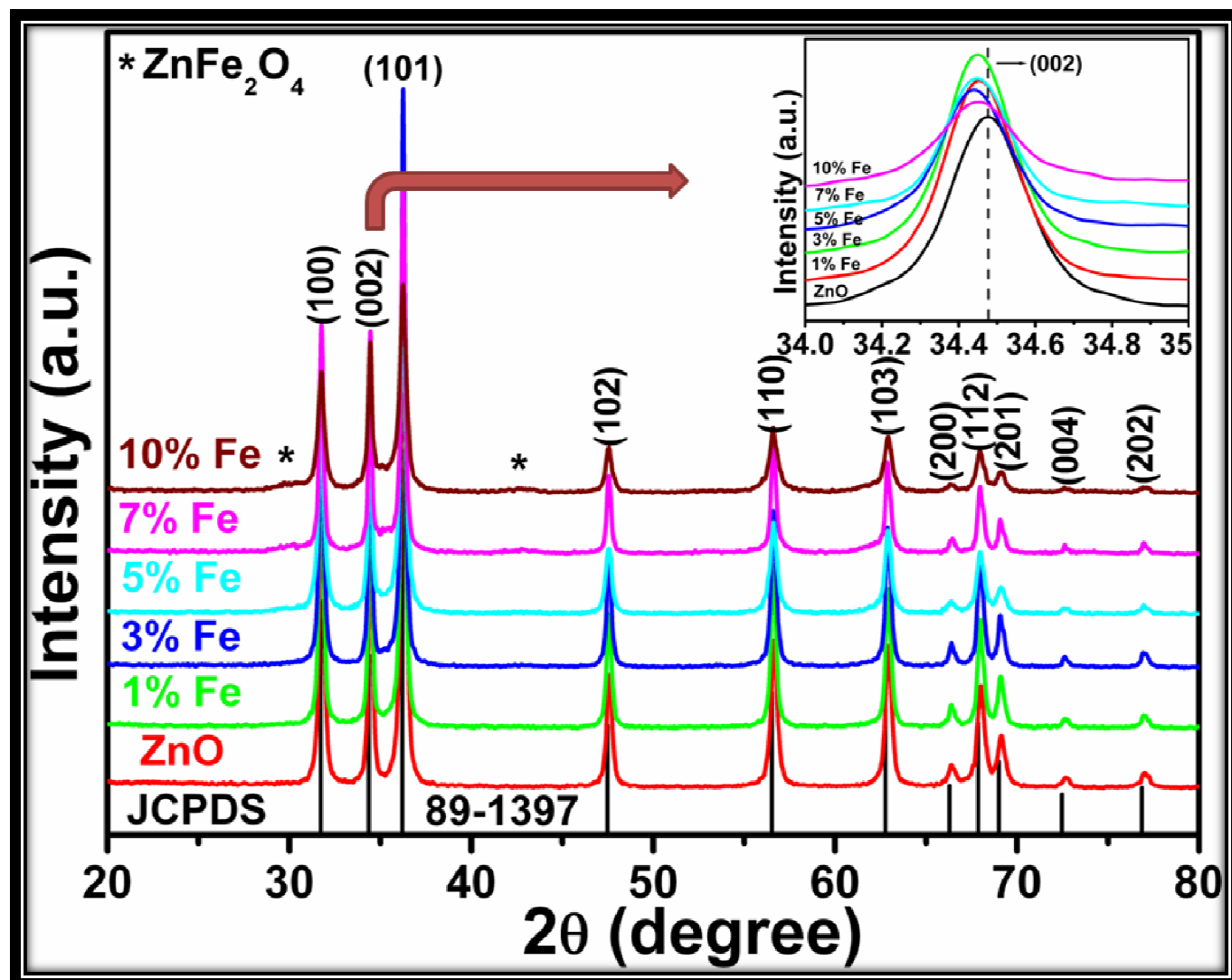
Fig. S1. XRD pattern of Zn 1-x Fe x O (0.0 ≤ x ≤ 0.10) nanostructures. Inset shows the magnified view of (002) peak depicting the shifting of peaks with Fe doping.
