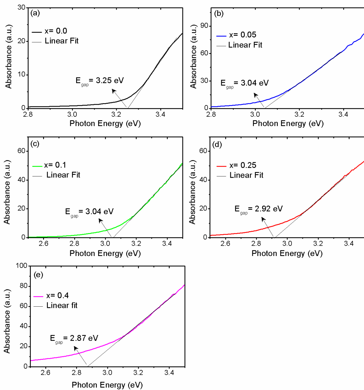
Figure 1S: UV-vis spectra dependent of the absorbance for the SrTi 1-x Fe x O 3
