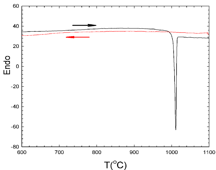
The DSC curve of \text{Ba}_2\text{Mg}(\text{B}_3\text{O}_6)_2 .
