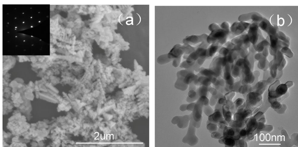
Figure S2 images of the \text{SrTiO}_3 dendrites synthesized at 180^\circ\text{C} for 36 h in 3 M NaOH solution: (a) FESEM image and the corresponding SAED pattern (inset), (b) TEM image.
