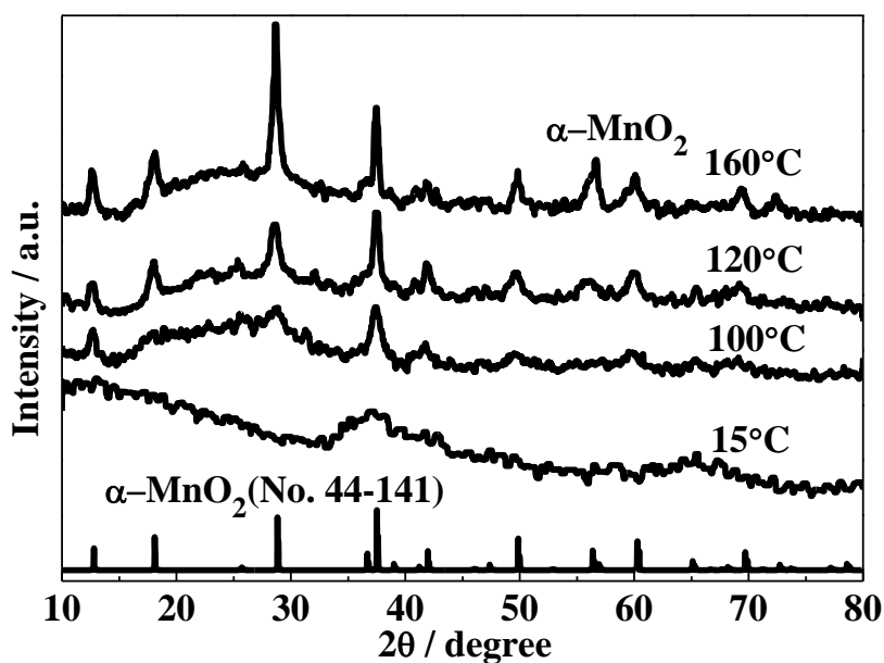
Fig. S1. XRD pattern of \alpha -MnO 2 synthesized at different reaction temperature aged for 10 h.
