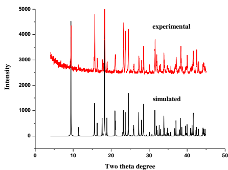
Fig. S1 The experimental and simulated powder XRD patterns for the title compounds.
