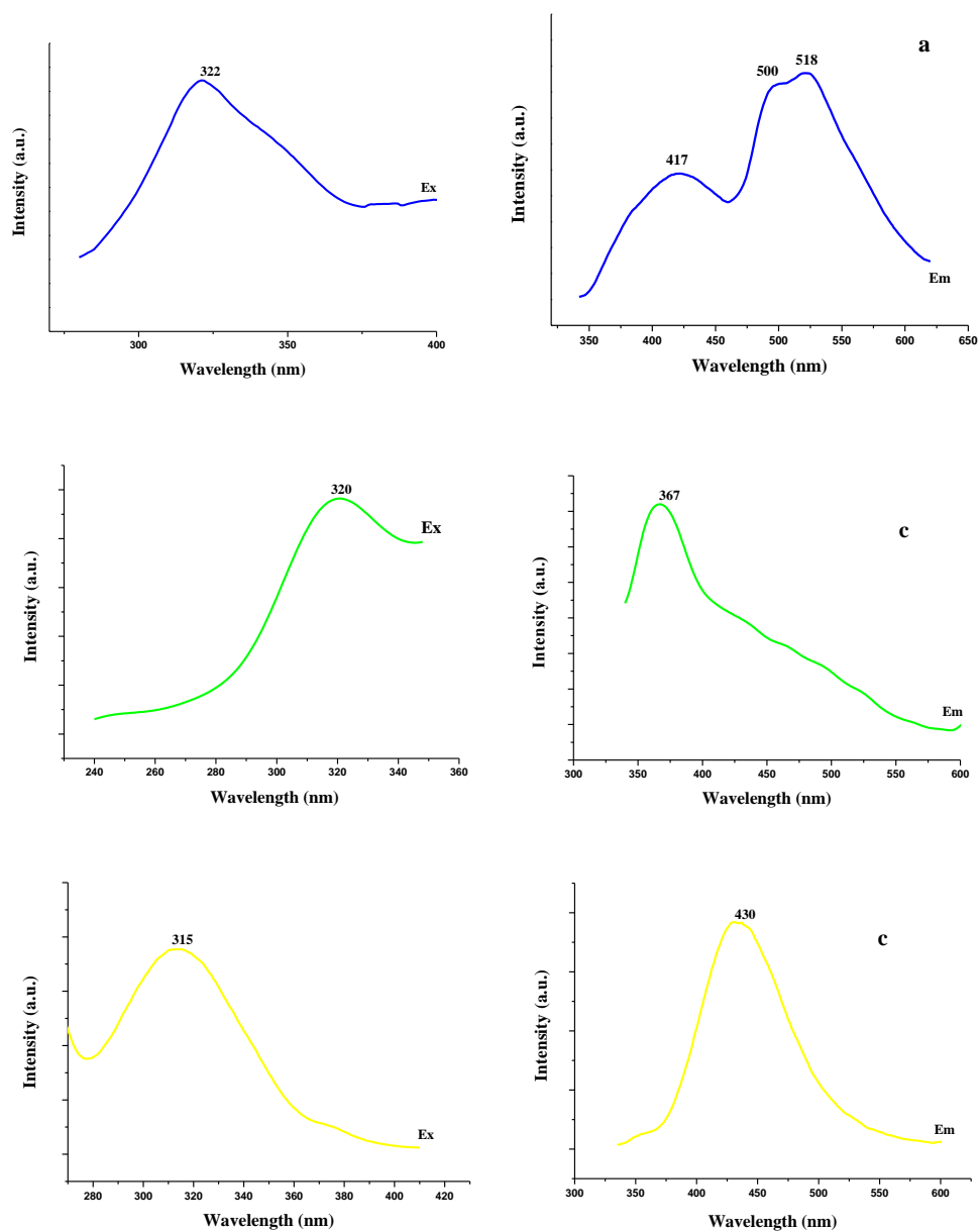
Fig. S3 The luminescence excitation and emission spectra of CdBr 2 (a), bpp (b) and dach (c).
