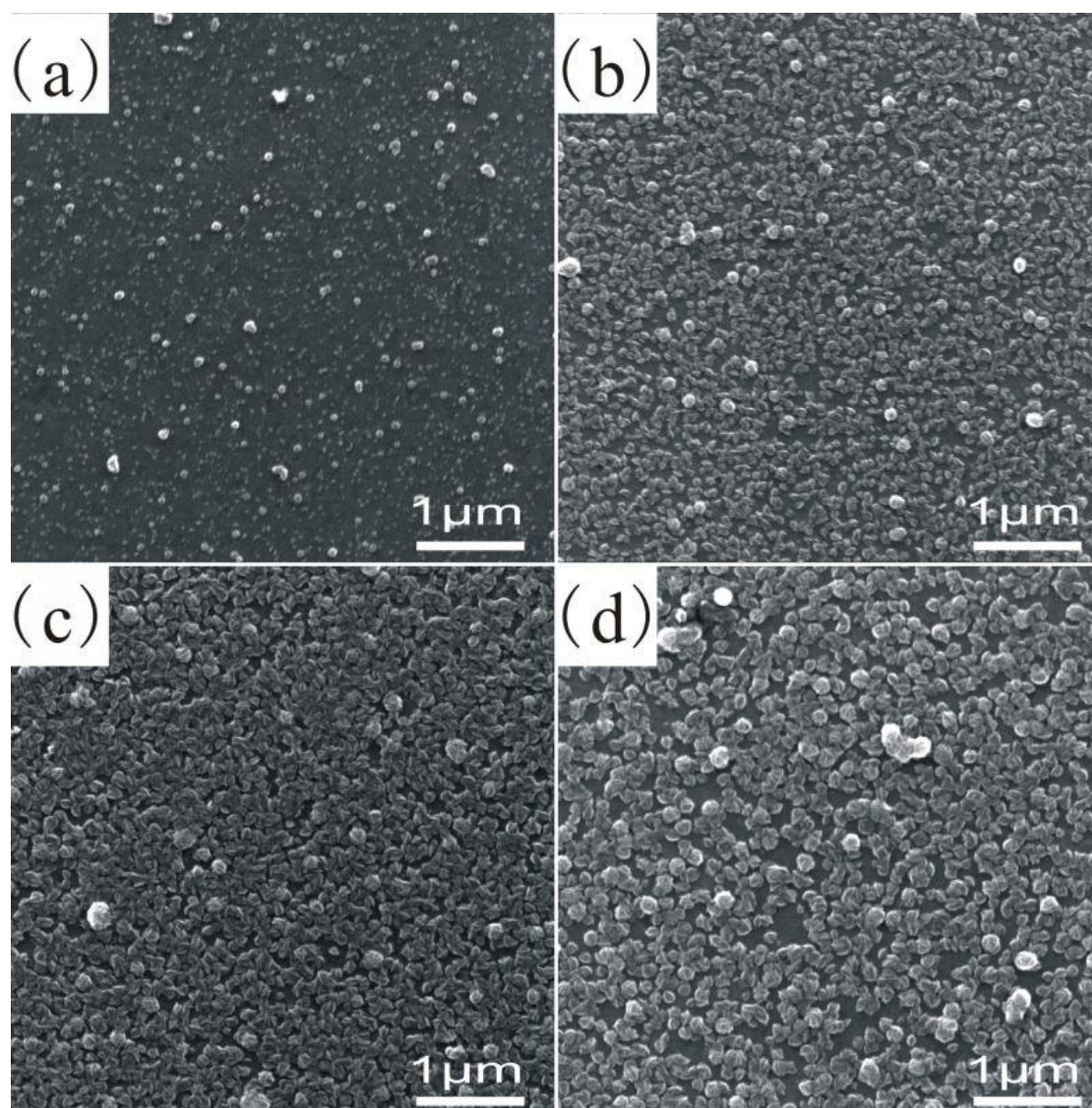
Figure S1. SEM images of CBD-grown CdS films on ITO substrates deposited at 50 °C with various deposition time: (a) 0.5 hour, (b) 1 hour, (c) 2 hours, (d) 3 hours.
