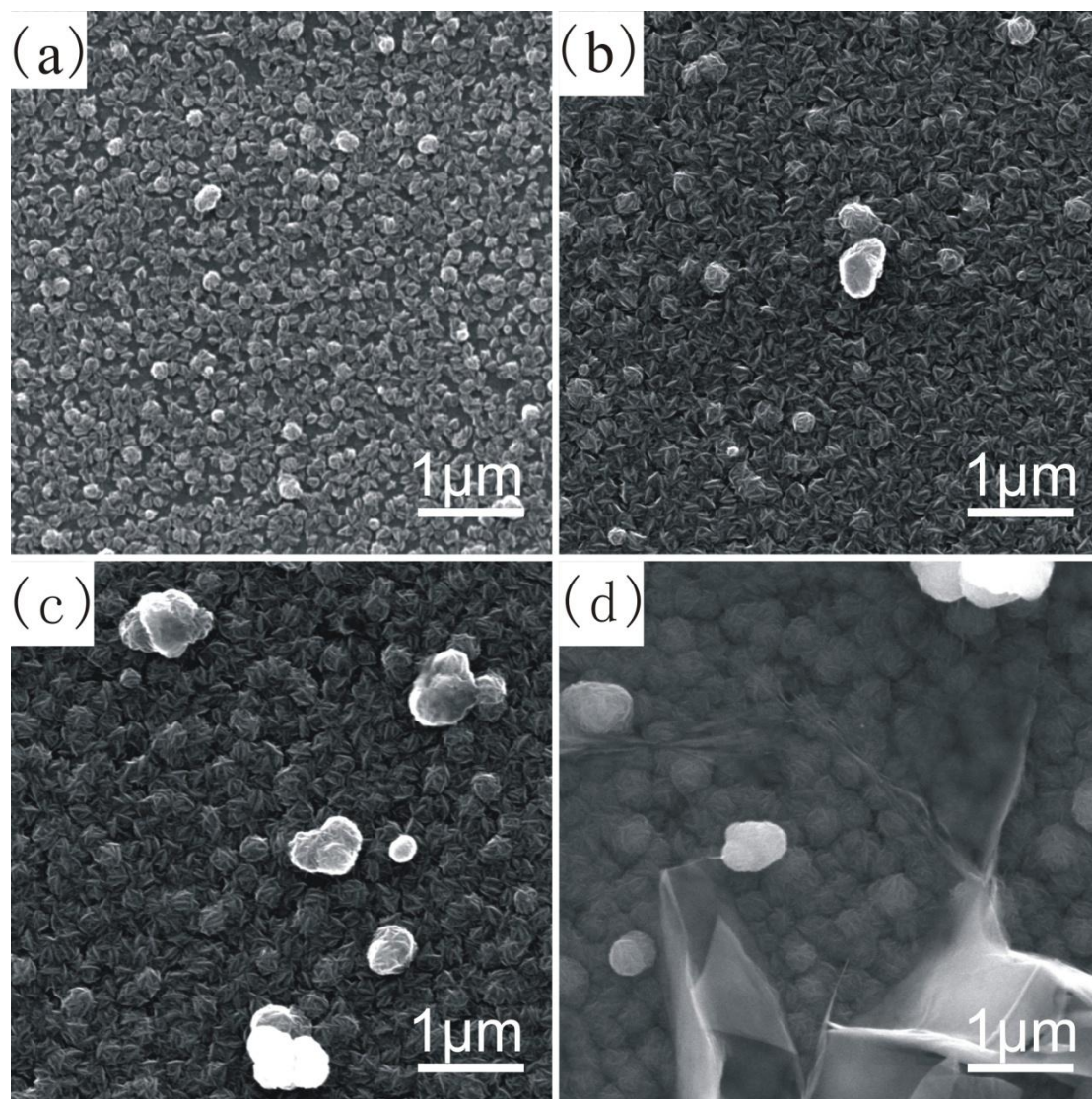
Figure S2. SEM images of CBD-grown CdS films on ITO substrates deposited at 80 °C with various deposition time: (a) 0.5 hour, (b) 1 hour, (c) 1.5 hours, (d) 2 hours.
