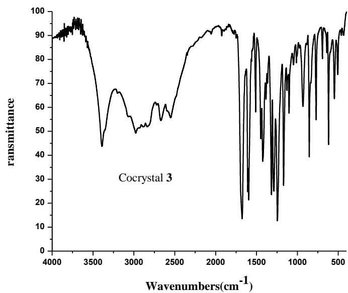
Fig. S1 Infrared spectra of cocrytals 1-3.
