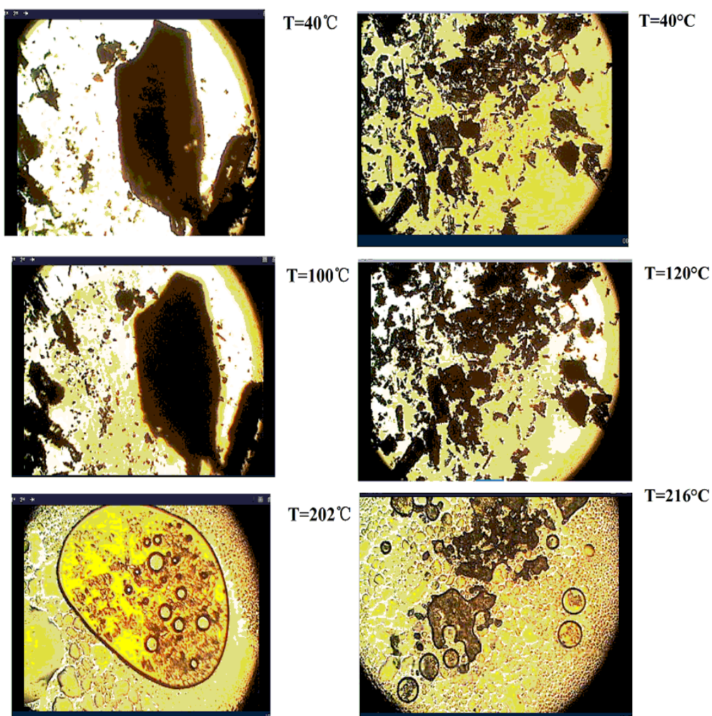
Fig. S2 Hot stage microscopy for cocrytals 2 (left) and 3 (right).
