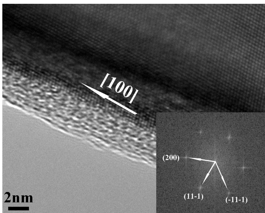
Fig S1. HRTEM image of an individual SiNW prepared by Ag-assisted chemical etching method. Inset shows the corresponding FFT pattern.
