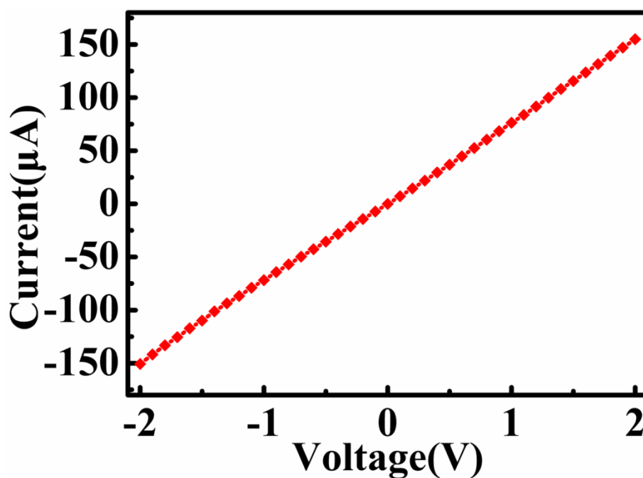
Fig S2. Typical I-V curve of p -CdTe :Sb NR.
