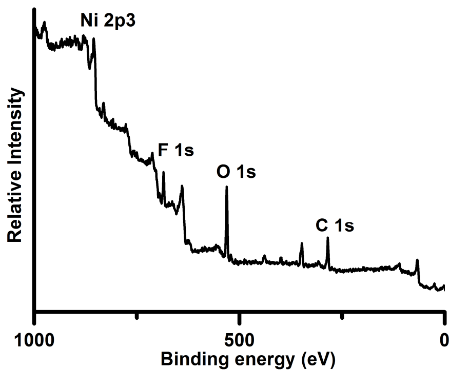
Fig. S2 XPS spectrum of nickel products obtained at 6 h.
