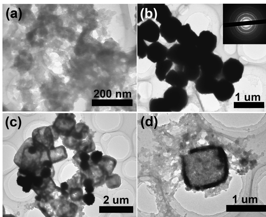
Fig. S1 TEM images of as-prepared products with the reaction time of (a) 1 h; (b) 2 h, inset: SAED pattern of a nickel cube; (c) 4 h; (d) 12 h.
