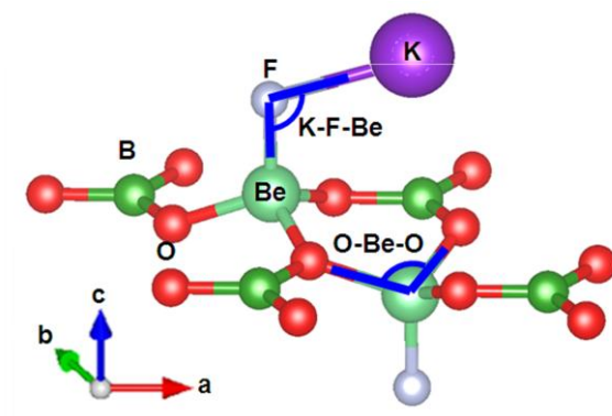
Figure S3. The sketch of the geometric relation between bonds and angles in layer (\text{Be}_2\text{BO}_3\text{F}_2)_\infty
