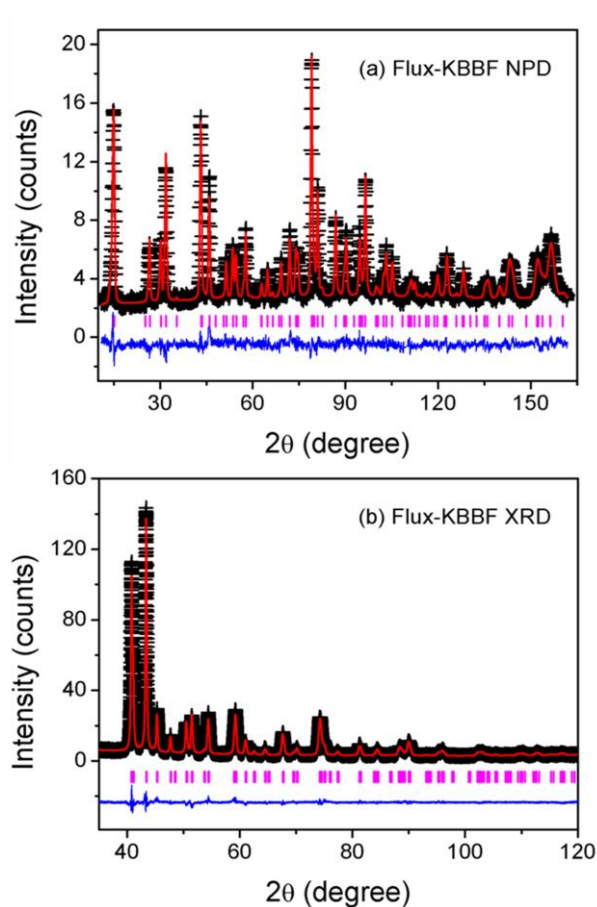
Figure S1. Combined Rietveld analysis of NPD (a) and XRD (b) for flux-KBBF powder. Plus (+) marks represent the experimental results and the solid line is from refinement. The ticks indicate the expected positions for structure R32 . The difference between experimental and calculated results is shown beneath.
