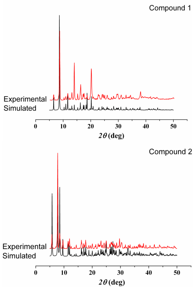
Fig. S2. Powder X-ray diffraction patterns of compounds 1 and 2
