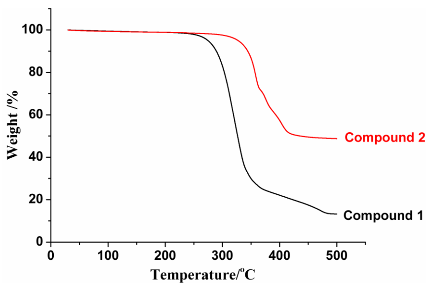
Fig. S1 TGA curves of compounds 1 and 2
