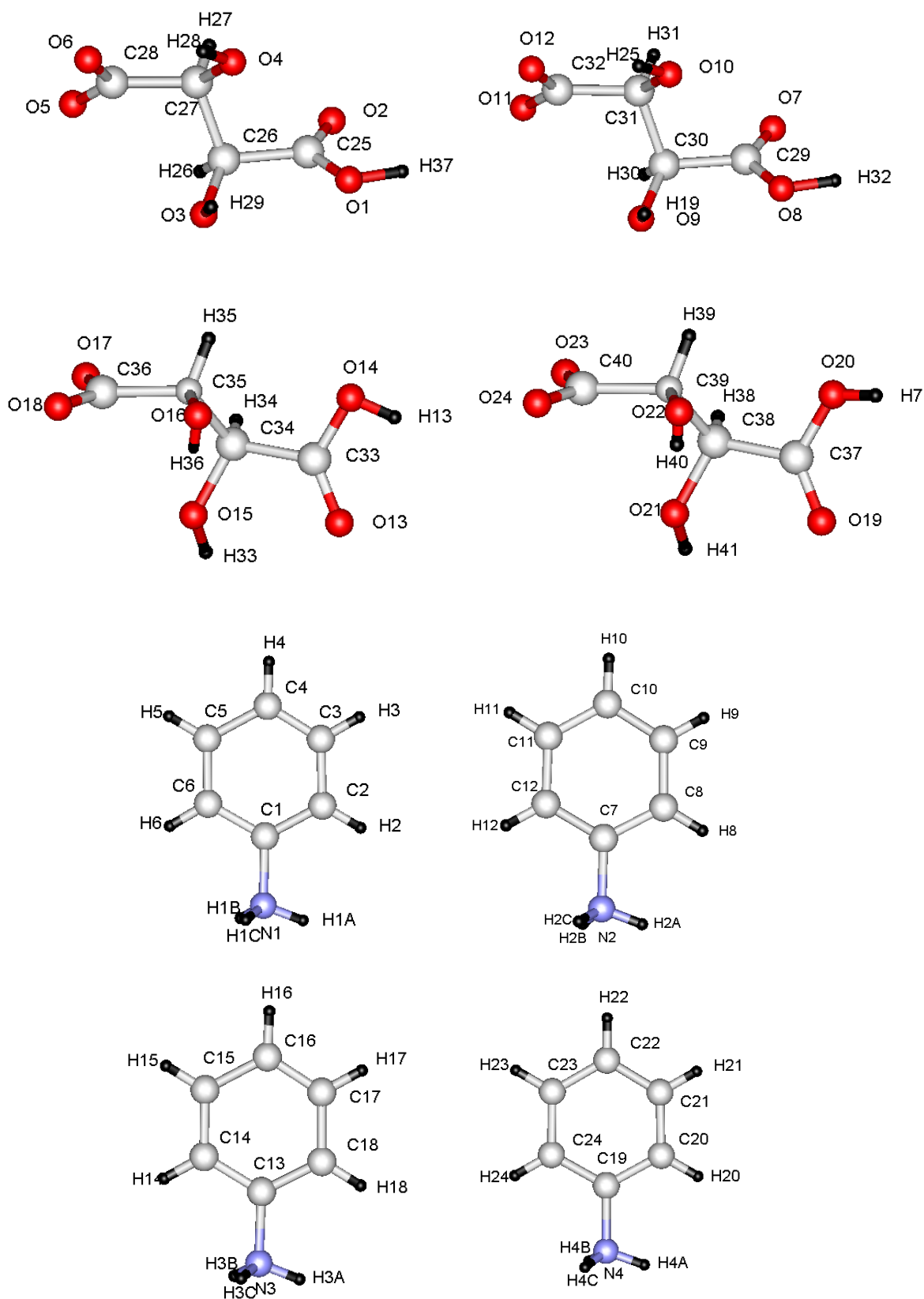
Figure S4. Atomic numbering scheme of (\text{Ani}^+)(\text{L-HTart}^-) at 300 K.
