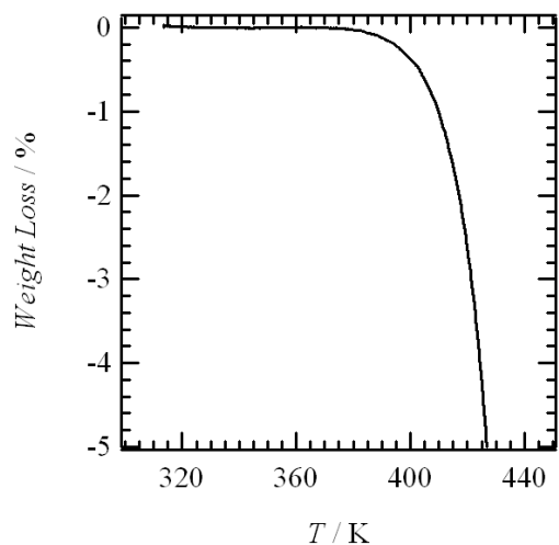
Figure S1. TG diagram of (\text{Ani}^+)(\text{L-HTart}^-) at the temperature range from 320 to 450 K.
