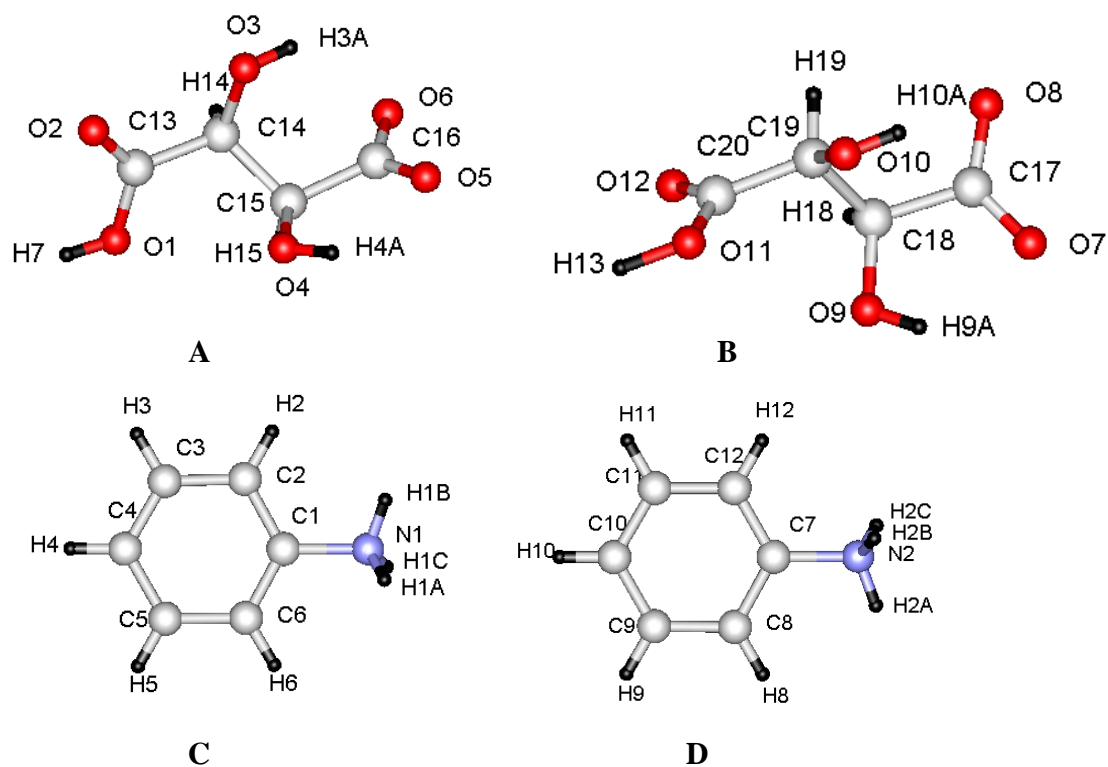
Figure S2. Atomic numbering scheme of (\text{Ani}^+)(\text{L-HTart}^-) at 100 K.
