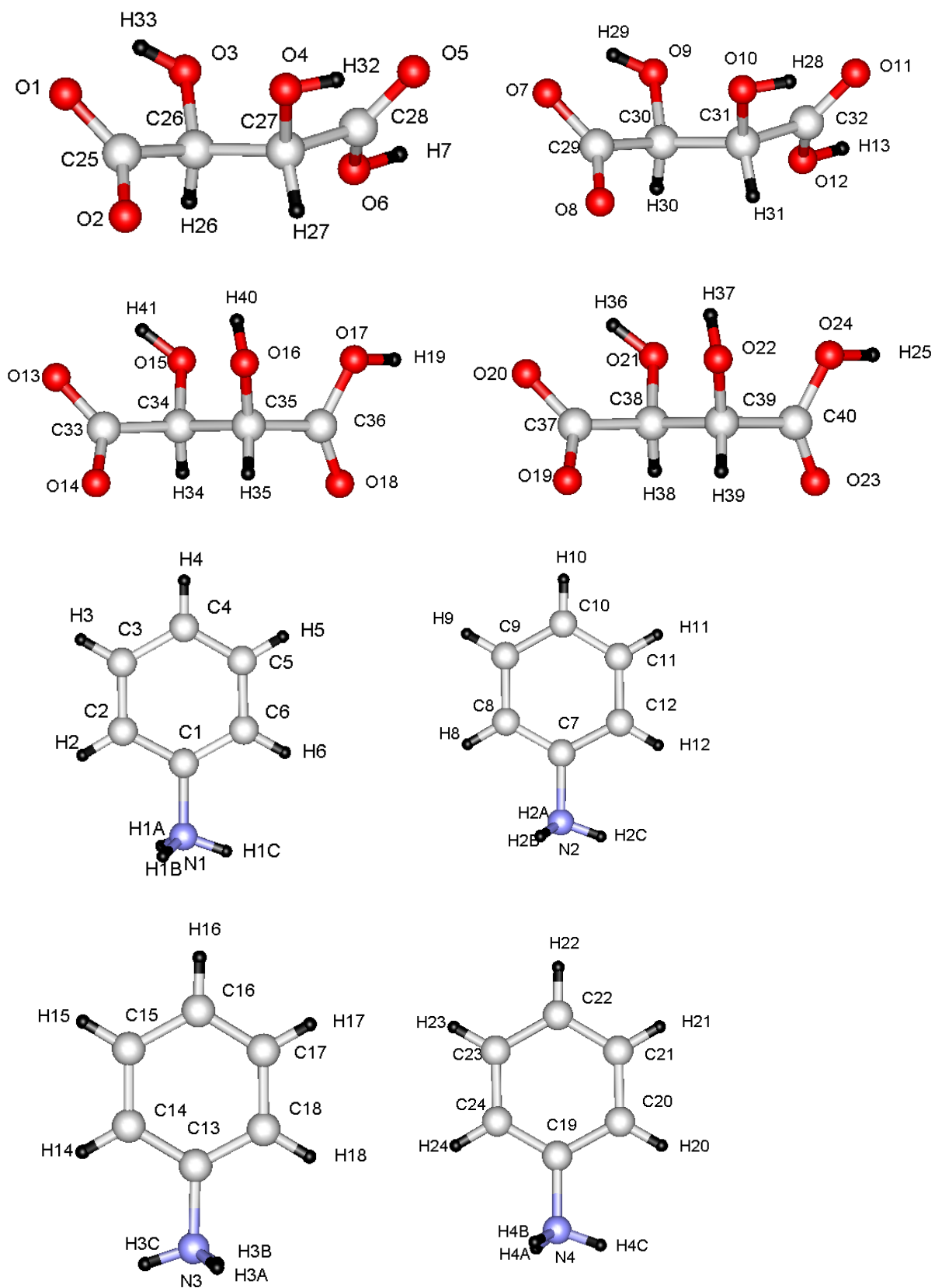
Figure S3. Atomic numbering scheme of (\text{Ani}^+)(\text{L-HTart}^-) at 250 K.
