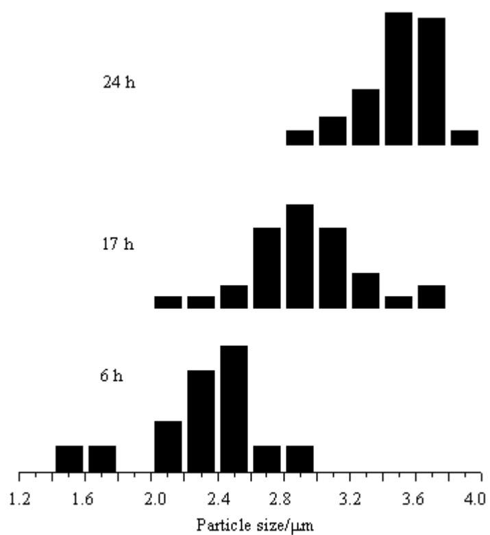
Fig. S1. The histogram of particle size distributions of obtained materials at different treatment times.
