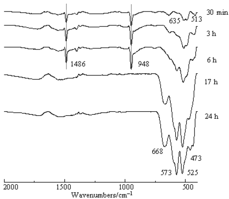
Fig. S2. IR spectra of the obtained materials at different hydrothermal treatment times.
