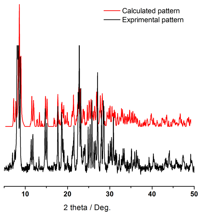
Fig. S2 The powder X-ray diffraction patterns and the simulated patterns of complex 1 .
