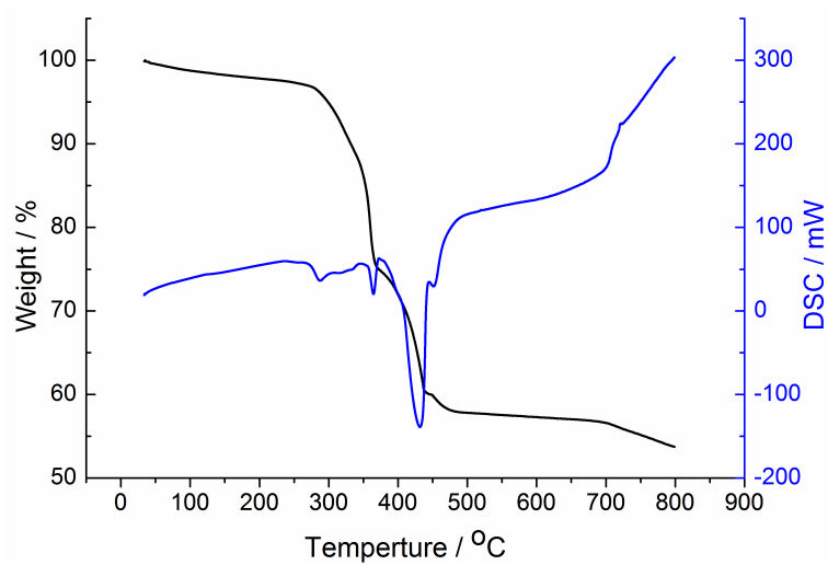
Fig. S3 TGA and DTA curves of complex 1 .
