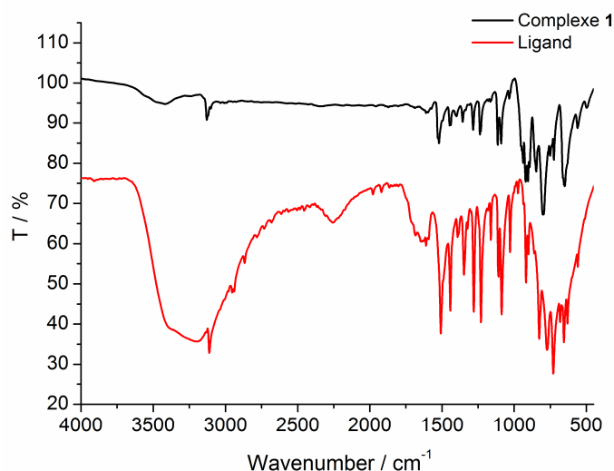
Fig. S1 The FT-IR spectra of ligand and complex 1.
