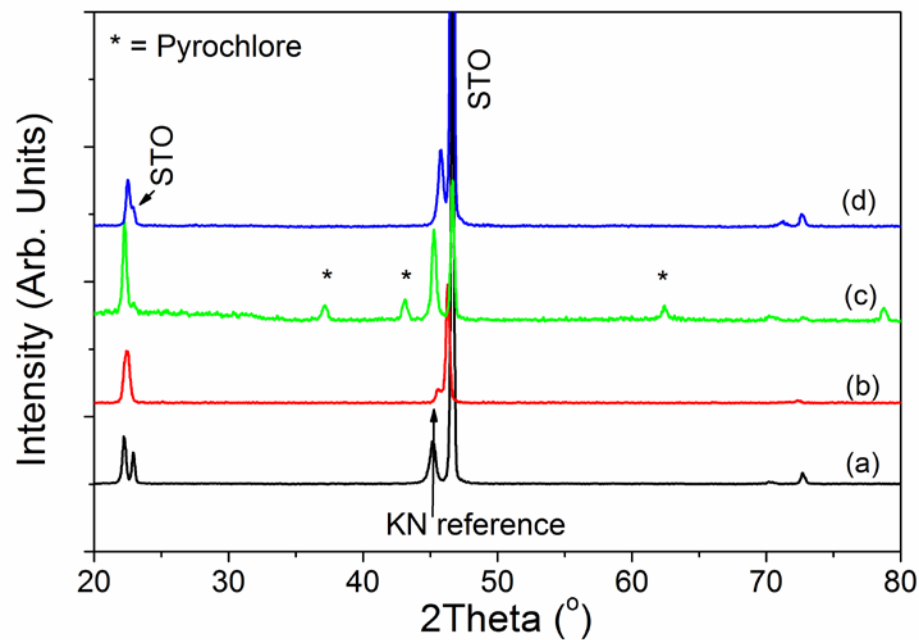
Supporting Figure 1: Full XRD scan range of manuscript Fig. 2 (a)
