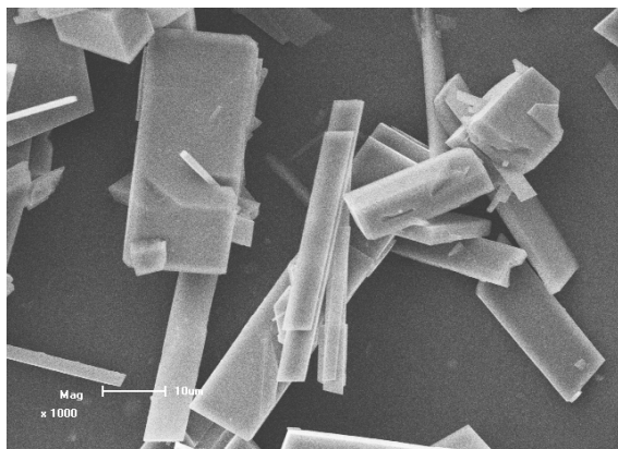
SEM image of \text{AlPO}_4\text{-34FF} crystals obtained from mixing solvent with thin strips morphology.
